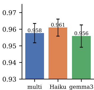
cosine EN↔back-transl.
