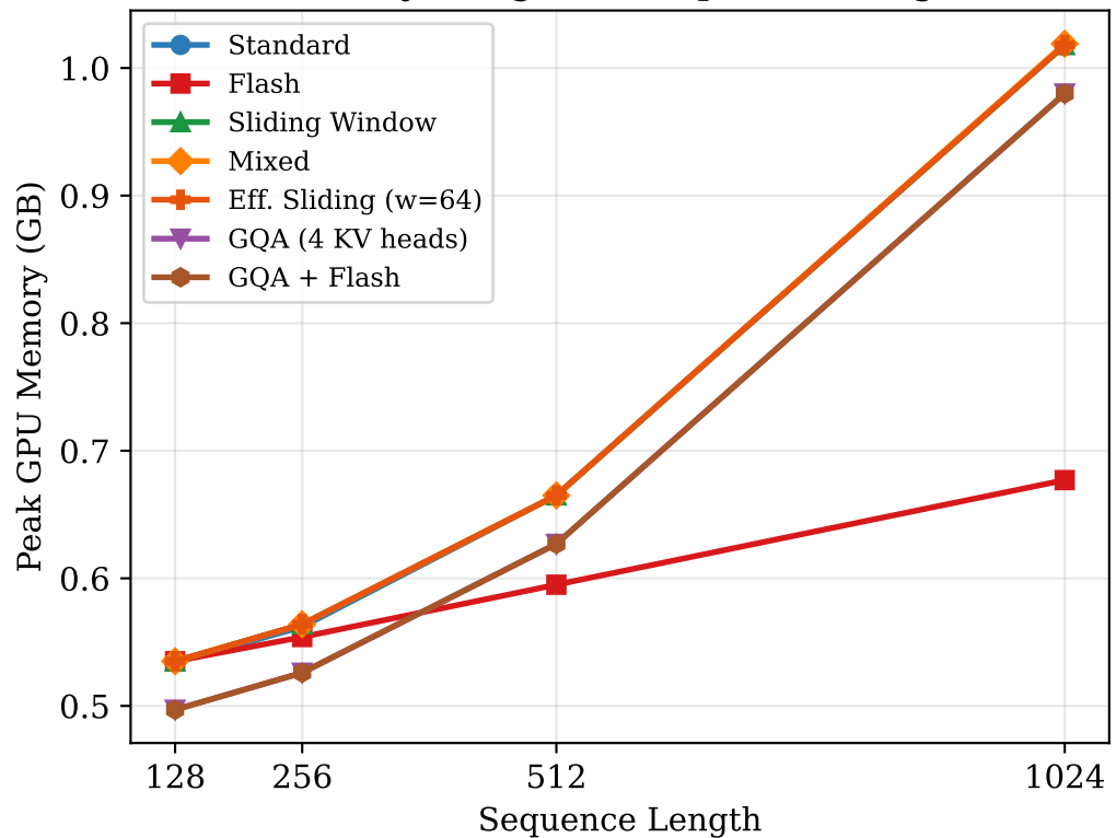
Memory Usage vs. Sequence Length
