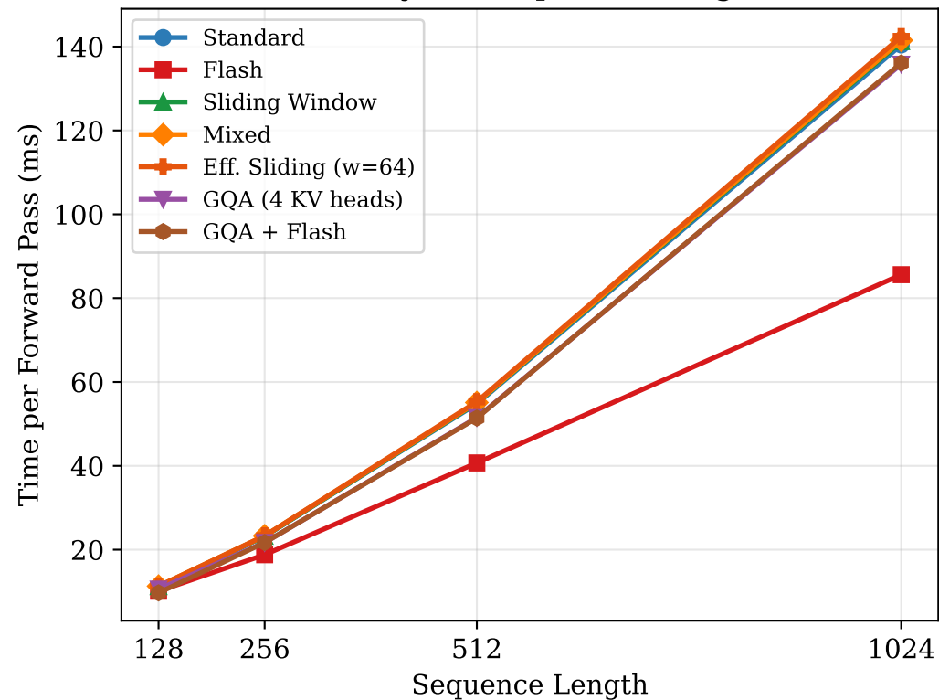
Latency vs. Sequence Length
