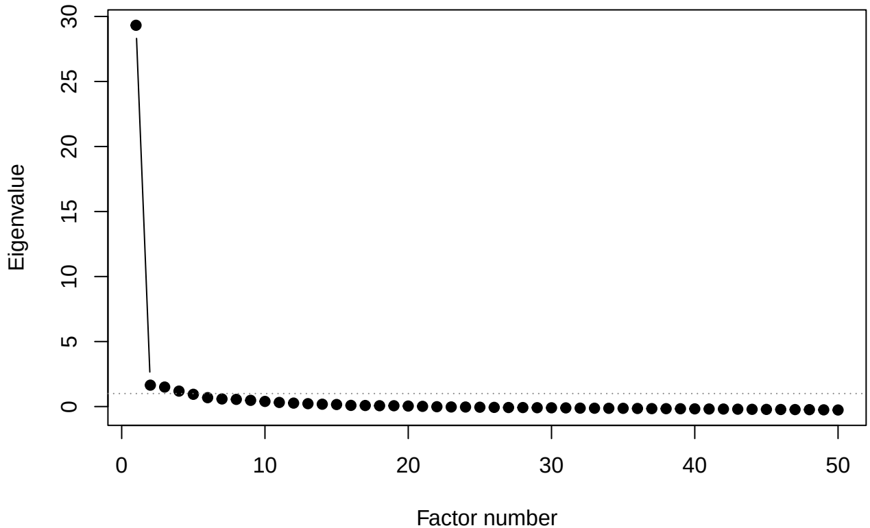
Scree plot with parallel analysis threshold
