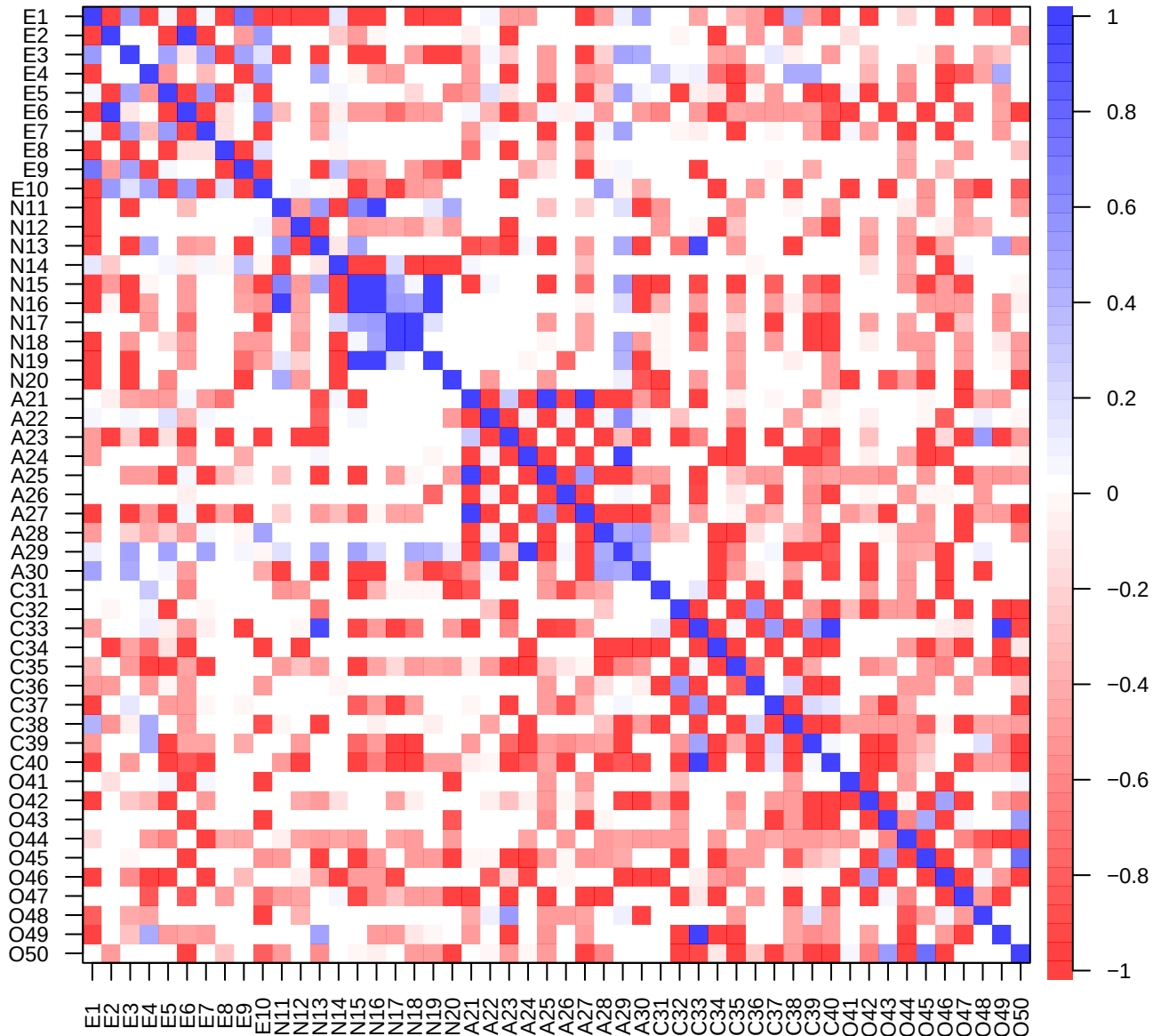
Correlation plot
