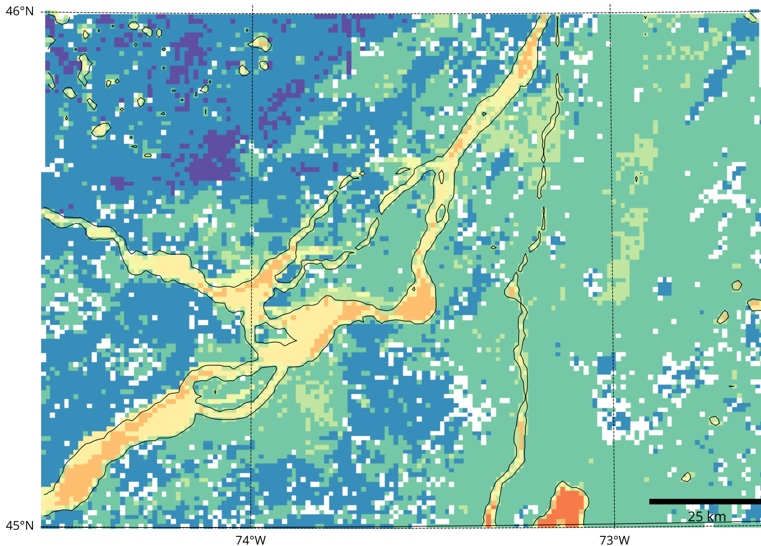
TEB+CLASS Upwards Surface Latent Heat Flux Anomaly During Observed Heat Wave Days
