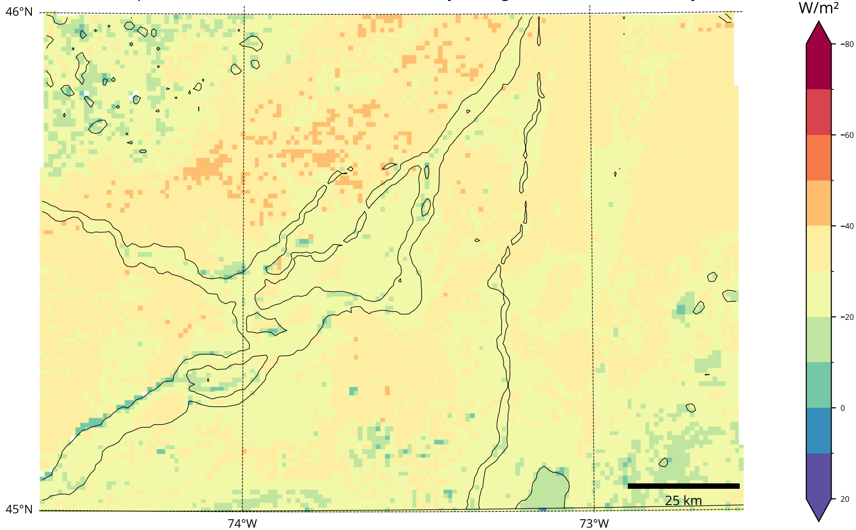
CLASS Upwards Surface Sensible Heat Flux Anomaly During Observed Heat Wave Days
