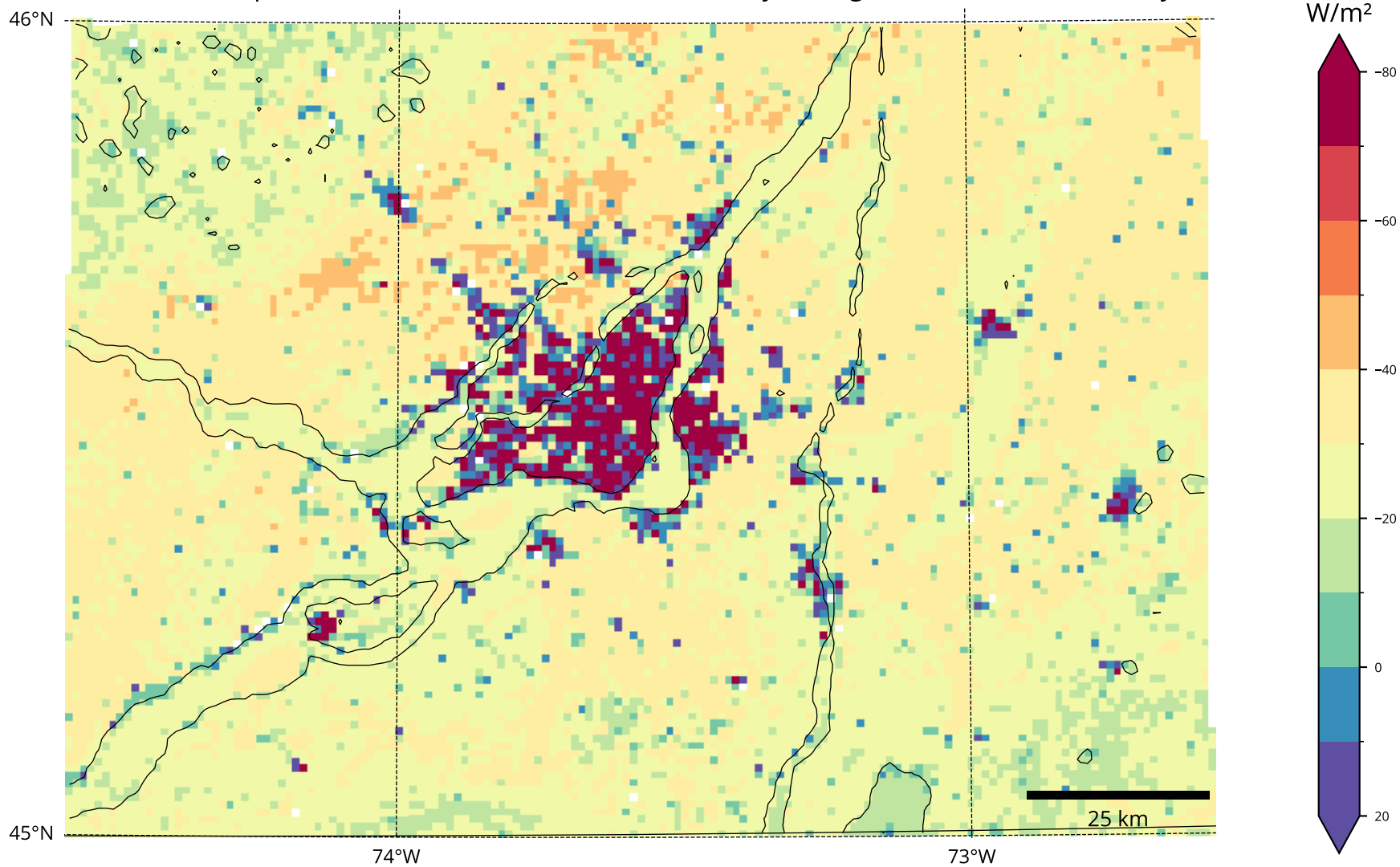
TEB+CLASS Upwards Surface Sensible Heat Flux Anomaly During Observed Heat Wave Days
