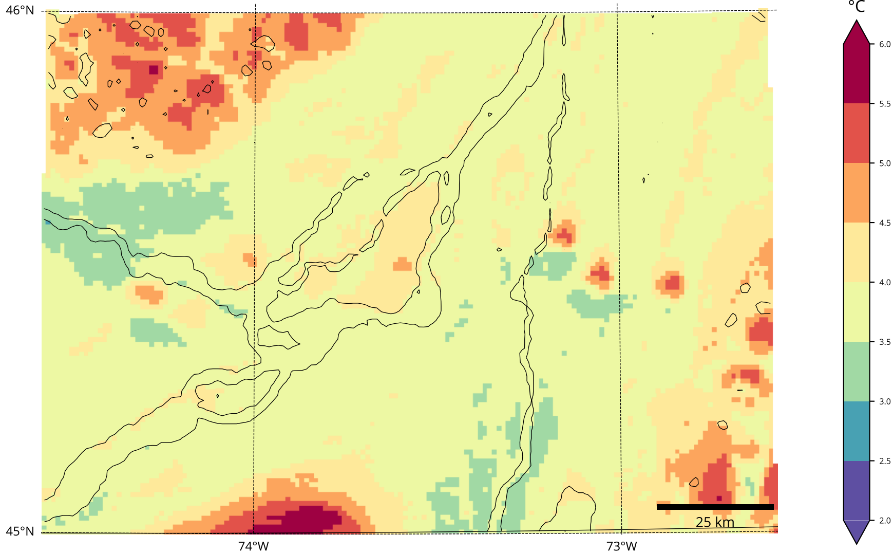
CLASS Minimum Daily 2m Temperature Anomaly During Observed Heat Wave Days
