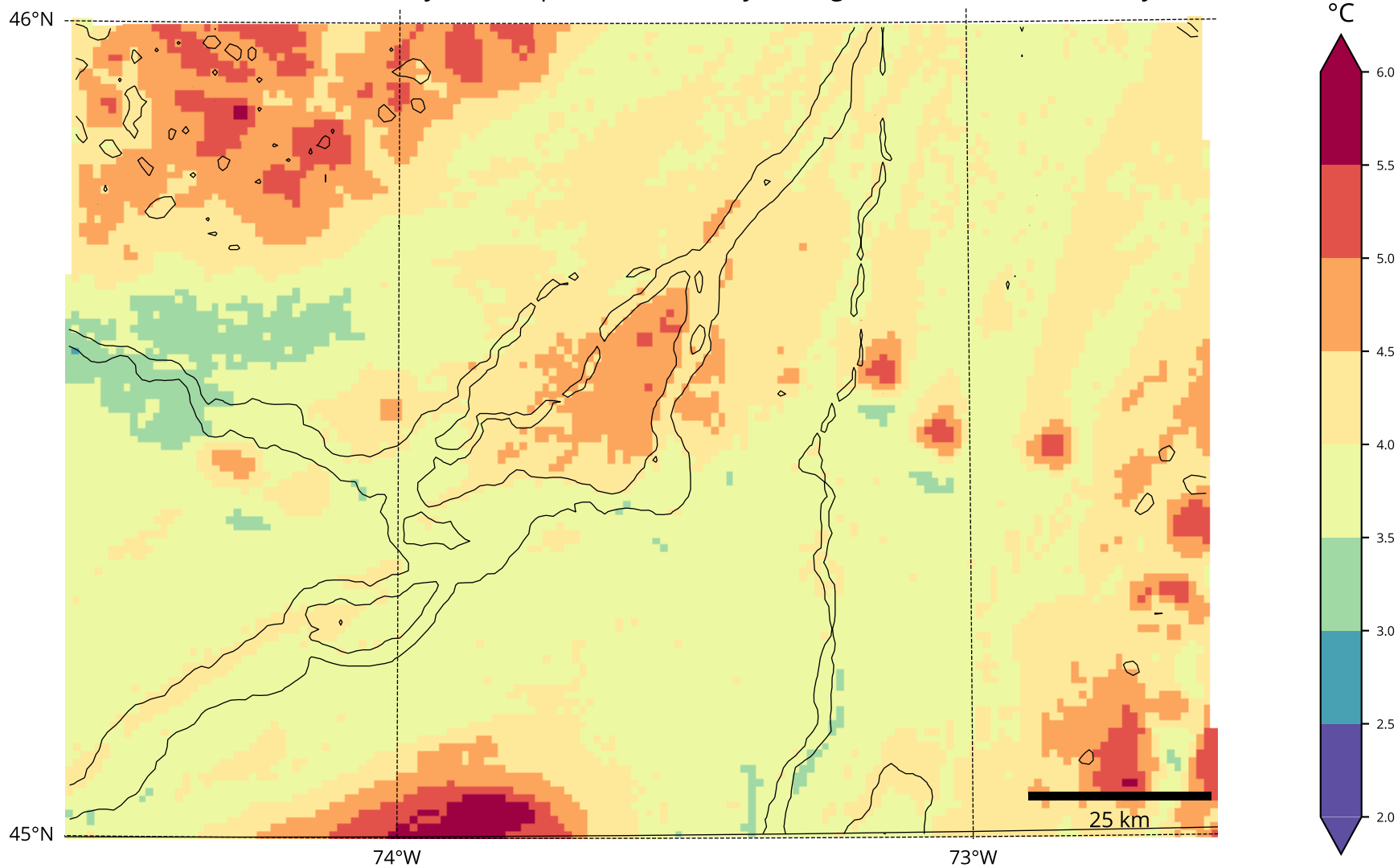
TEB+CLASS Minimum Daily 2m Temperature Anomaly During Observed Heat Wave Days
