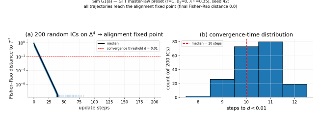
Figure S2. Sim G1(a): convergence to the alignment fixed point from 200 random initial conditions on \Delta^4 (planted \lambda = 0.35 ). Fisher–Rao distance trajectories and convergence-time histogram: final distance 0.0 for all trajectories, median 10 steps to d < 0.01 (§3.6).
