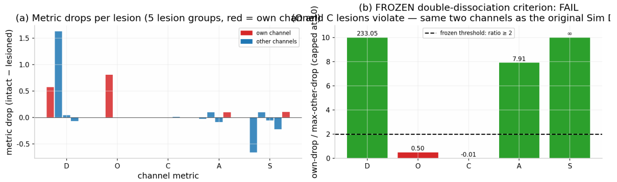
Figure 23: Sim D10 E2 lesion battery under the frozen double-dissociation criterion (verification re-run, seed 42). The criterion fails as frozen, as in the original run (own-channel degradation ratios in this reconstruction: D 233 \times , A 7.9 \times , S unbounded; O 0.50 and C -0.01, both failing); the post-hoc cascade edges are labeled on-figure as hypothesis-generating only.
