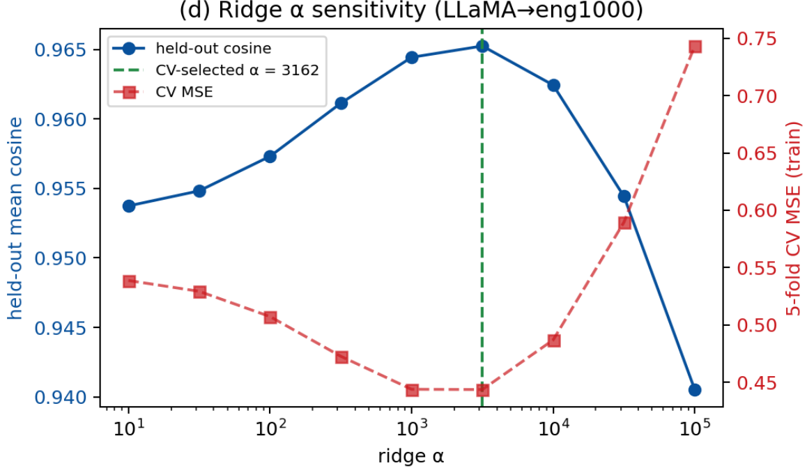
Figure 20: Bridge regularization selection (§5.2). 5-fold CV MSE over \alpha \in \{10^1 \dots 10^5\} on the 512 training pairs; selected \alpha = 3162 for LLaMA \rightarrow eng1000, refit on the full training set.
