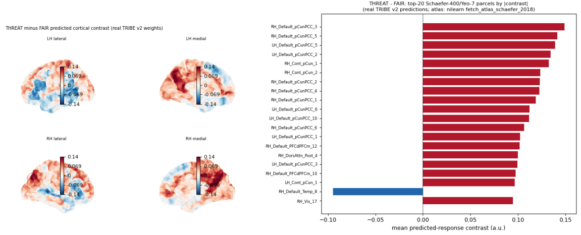
Figure 7: Submission re-run, THREAT-FAIR vertex-wise contrast (reconstructed stimuli; descriptive contrast, not an inferential statistic). Left: contrast rendered on fsaverage5 pial surfaces (4 views). Right: top-20 Schaefer-400 parcels by |\text{contrast}| — 16 of 20 are Default-mode (Default_pCunPCC dominant) or Control network parcels, the same network family as the main-text localization, with exact parcels differing across the different texts.
