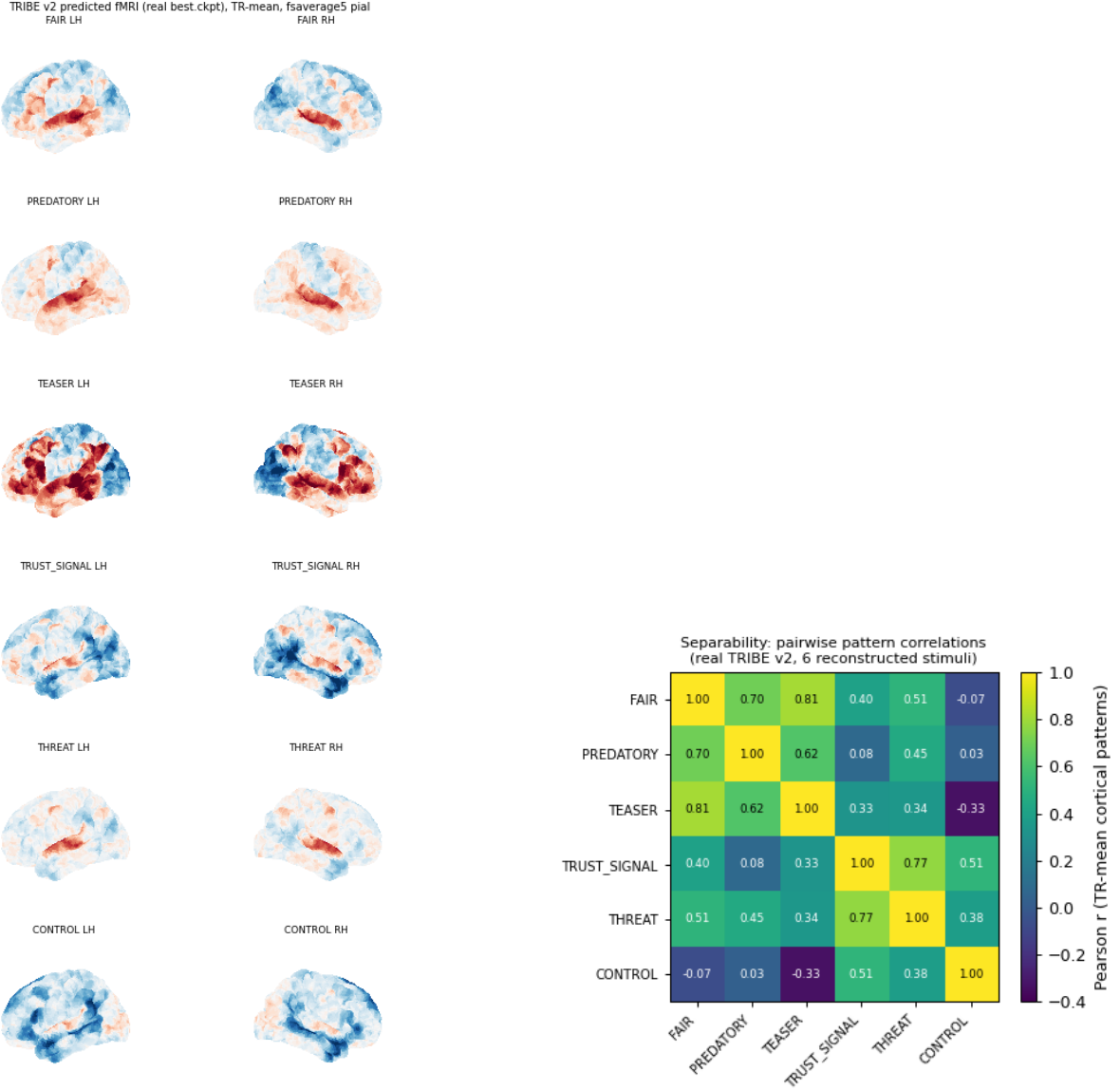
Figure 6: TRIBE v2 submission re-run (official Python reference; deterministic; §5.2; reconstructed offer-category stimuli with uniform word timing, the verbatim §M texts bundled with the Supporting Document (deposit pending)). Left: TR-mean predicted cortical response per stimulus (six categories, lateral views on the real fsaverage5 pial mesh). Right: pairwise Pearson similarity of the TR-mean patterns — every pair distinct ( r from -0.33 to +0.81 , all cleanly below 1.0), a qualitative reproduction of the separability claim; values sit below the verbatim-stimulus battery’s 0.82–0.99 because the stimuli are reconstructions, not the originals.
