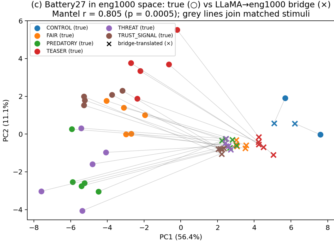
Figure 19: Battery27 downstream in eng1000 space via the bridge (same reconstruction-from-spec label as Figure 9). PCA of true eng1000 features vs. LLaMA features translated through the ridge map: translated-vs-true per-item cosine 0.813 (tight null 0.791, p = 0.0005 ); RDM Mantel r = 0.805 , p = 0.0005 (raw un-translated LLaMA RDM: r = 0.362 — the bridge doubles the geometry match); category LOO decode 1.00. The ridge’s regression-to-mean shrinkage toward the centroid is visible, and exact-item retrieval among the 27 is at chance because same-category items are near-duplicates in true eng1000 space itself; category-level geometry — what the pipeline consumes — is preserved.
