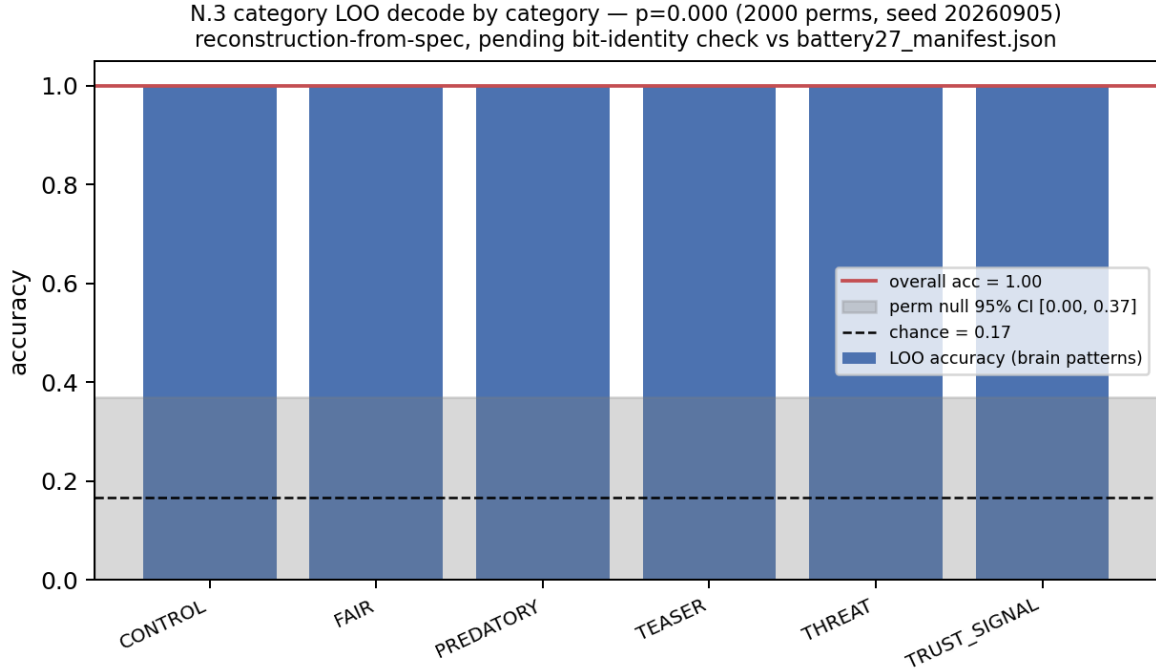
Figure 15: Extended battery, N.3 Gallant-style decode with the real Huth-lab english1000 985-dimensional semantic model (OpenNeuro ds003020 derivatives; same matrix as Huth et al. 2016) (same reconstruction-from-spec label as Figure 9; 2,000 permutations per null, seed 20260905, leave-8-out folds). Ridge encoding generalizes (mean vertex r = 0.181 , p = 0.0005 , resolution-limited at 2,000 permutations); exact stimulus retrieval is NULL (top-1 0.037, p = 1.0 ) and Procrustes alignment is NULL ( r = -0.058 , p = 0.769 ) — matching the original battery’s reported null pattern (reference only). Category leave-one-out decode is perfect (1.000, p = 0.0005 ) but is driven by the reconstruction’s templatic within-category lexicon — the semantic-only control decodes at 1.000 too — and is explicitly NOT comparable to the original battery’s 0.40.
