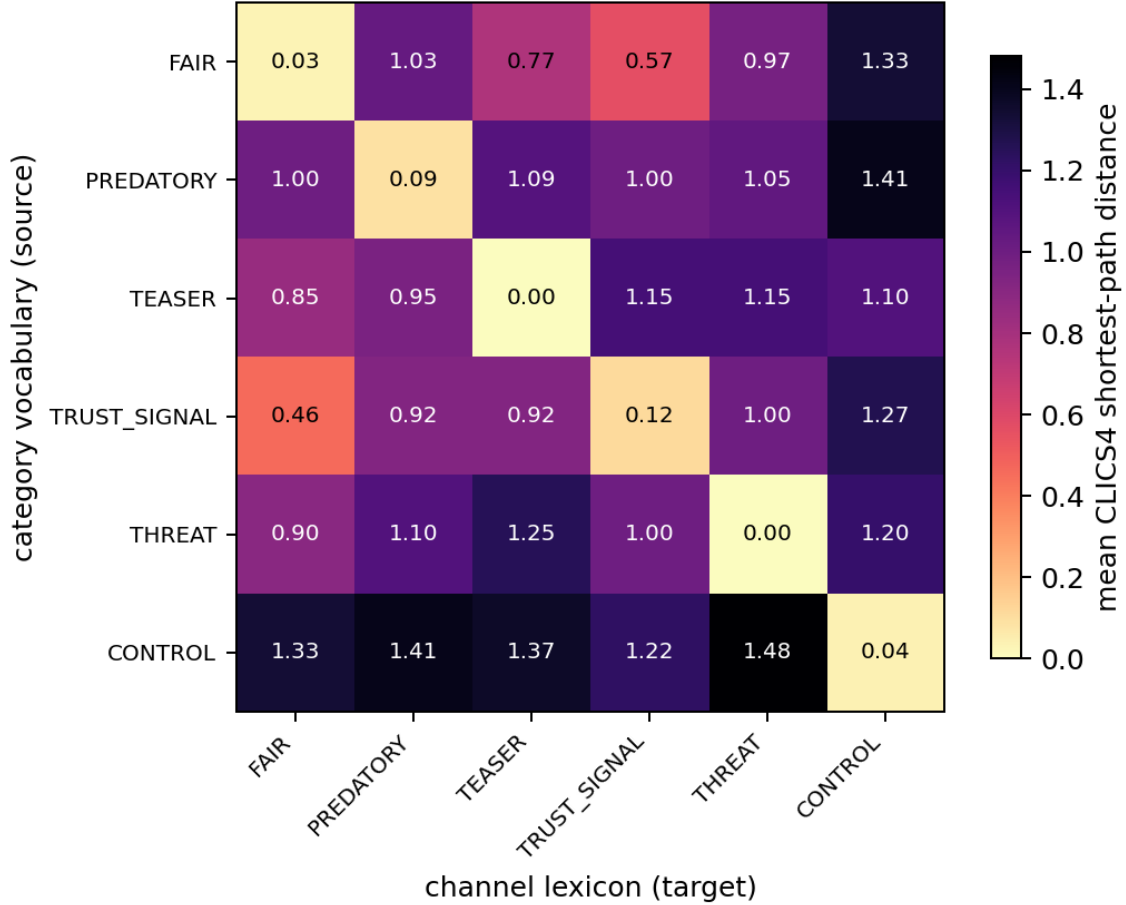
N.4 CLICS4 colexification distances: category vocabulary -> channel lexicons .ICS4 graph, 51,562 edges; reconstruction-from-spec, pending bit-identity check vs battery27_nr
