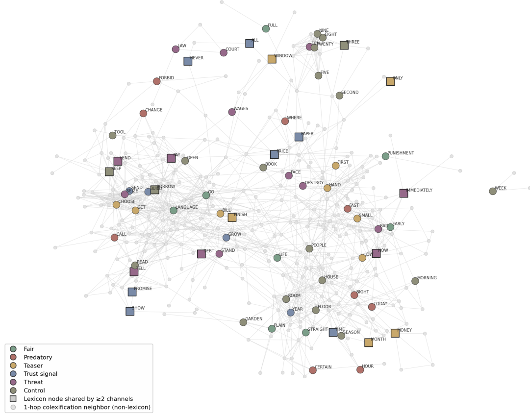
Figure 3: CLICS4 colexification neighborhoods of the six channel lexicons (§4.6; real CLICS4 CLDF data, Family_Count \geq 3 filter: 1,386 concepts / 3,986 edges — re-verified, matching the §4.6 sensitivity row; the 51,562-edge unfiltered graph is too dense to render legibly). Spring layout (seed 42): 75 mapped lexicon concept nodes (colored by channel; squares = nodes shared by \geq 2 channels) plus their 1-hop colexification neighbors (grey), 393 nodes / 1,196 edges. Lexicon membership and the exact/morphological/synonym Concepticon mapping tiers are taken from the archived battery analysis; the channel lexicons are battery-derived (labeled on the figure), since the paper's own channel-concept lists are in the Supporting Document (deposited at OSF). Network style after the language-family networks of Jackson et al. (2019).
