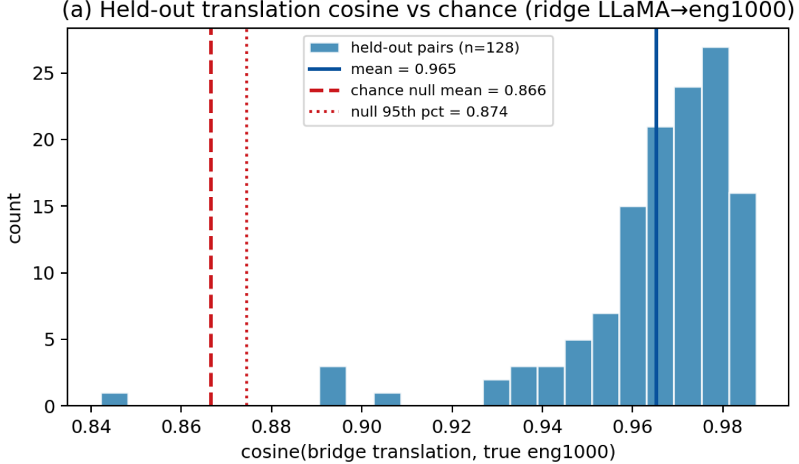
Figure 17: Supervised LLaMA → eng1000 ridge bridge (§5.2) — held-out cosine, reported only against its null ( N = 640 paired real NQ-corpus texts, 64-token chunks, eng1000 coverage \geq 0.5 ; 512 train / 128 held-out; seed 42; ridge \alpha = 3162 by 5-fold CV). Held-out paired mean cosine 0.965 vs. random-pairing null mean 0.866 (null p95 0.874); permutation p = 0.0005 (2,000 reps). The null is high because eng1000 is anisotropic — the signal is paired \gg null, not the absolute cosine value.
