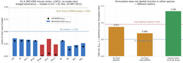
Figure 25: Simulation H1 on MICrONS mouse cortex. Left: dominant input class share per post class (bars), with the same class’s availability among pre-synaptic partners (black diamonds); red bars mark the three self-recurrent classes whose dominance exceeds availability by more than the A2 gap tolerance (0.15). The A1 criterion line (0.50) and the fly Kenyon-cell budget share (0.982, dotted) are shown for scale — no cortical class approaches either. Right: non-abolition under global partner permutation, on incommensurable metrics. The fly criterion-5 shuffles (F1a2: R_{\text{final}} 0.873 position-based; 0.680 class-faithful, where 1 = abolished, against a > 0.95 abolition requirement) fail, while mouse cortex under global partner permutation increases throughput ( R_{\text{perm}} = 1.340 against a \geq 0.50 retention requirement). Global partner permutation fails to abolish function in both species — on different metrics and criteria, not a matched quantitative replication; the structural basis differs.
