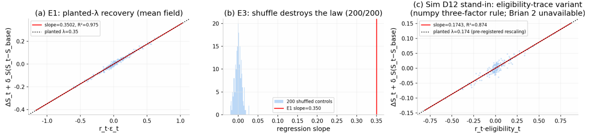
Figure 22: Sim D10 E1 planted- \lambda recovery (slope 0.3502 vs. planted \lambda = 0.35 , R^2 = 0.975 ), E3 shuffle negative controls (200/200 destroyed), and the Sim D12 numpy three-factor eligibility stand-in (planted 0.174 recovered as slope 0.1743, R^2 = 0.874 ).
