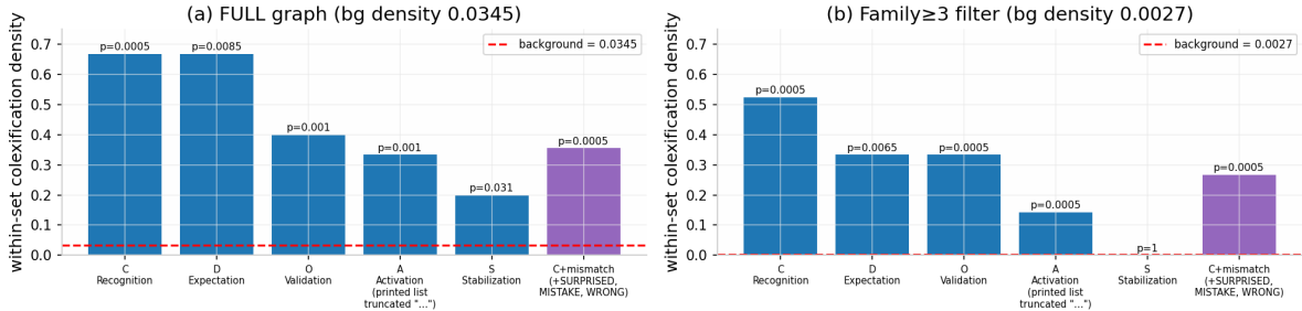
Figure 2: CLICS 4.0 within-channel colexification densities under the unfiltered and \geq 3 -family filters, with permutation p -values (2,000 permutations; re-run on the CLDF release, seed 42). The Recognition set reproduces the known perception \rightarrow cognition universal; the Stabilization set is a full null under the \geq 3 -family filter; the mismatch-augmented Recognition set passes ( p = 0.0005 ).
