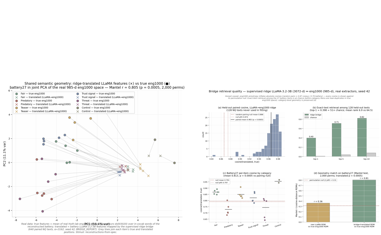
Figure 21: Bridge shared-latent geometry and retrieval summary (§5.2; real bridge results, seed 42; same reconstruction-from-spec battery label as Figure 9). Left: joint PCA (fit on the 54 stacked vectors) of true eng1000 battery features (dots) vs. ridge-translated LLaMA features (crosses), colored by battery category, with grey pairing lines; header carries the Mantel geometry match ( r = 0.805 , p = 0.0005 ). The translated cloud shrinks toward the centroid (ridge regression-to-mean) while category structure is preserved — exactly what the Mantel number quantifies. The true battery features were recomputed from the real english1000sm.hf5 (OpenNeuro ds003020 snapshot) with the exact pipeline code path; recomputed per-item translated-vs-true cosines match the archived bridge results to max |\Delta| = 1.2 \times 10^{-9} — a functional bit-check of the whole chain. Right: retrieval-quality panel — held-out cosine histogram (128 NQ pairs, mean 0.965) against the random-pairing null (mean 0.866 / p95 0.874; the anisotropy caveat is stated on the figure), top- k retrieval vs. chance, battery27 per-item cosine by category vs. the pairing null, and the Mantel geometry match (bridge 0.805 vs. raw-LLaMA 0.362 vs. null |r| p95 0.315).
