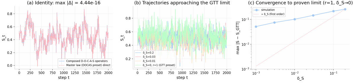
Figure 1: Operator composition and master-law verification (independent verification re-run, numpy, seed 42). The composed D \rightarrow O \rightarrow C \rightarrow A \rightarrow S operator loop reproduces the master-law DOCAS preset to machine precision ( \max |\Delta S| = 4.4 \times 10^{-16} over 2,000 steps), and the trajectories approach the theory’s physics-layer limit as \delta_S \rightarrow 0 , r \rightarrow 1 . Self-consistency check of the definitions; not evidence about biology.
