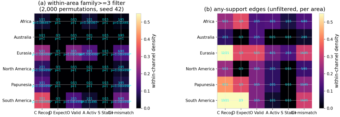
Figure 4: CLICS 4.0 per-macroarea subgroup analysis (SIM-R2 battery 7, seed 42; 51,562 edges, 1,725 concept nodes — re-run-verified counts): (a) within-area fam \geq 3 -filtered channel densities with hits/pairs and permutation p-values per Glottolog macroarea; (b) the unfiltered any-support panel at higher densities. S is null in all six macroareas; C is significant in 5/6 (Australia a power null); A is subgroup-positive in Africa and South America; D/O are underpowered per area (§4.6).
