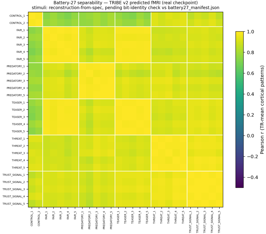
Figure 9: Extended battery, N.1 separability (§5.2; reconstruction-from-spec battery, pending bit-identity against battery27_manifest.json ): 27 \times 27 pairwise Pearson correlation of TR-mean predicted cortical patterns from the canonical pipeline (no-BOS LLaMA-3.2-3B, layers 17 & 24, 100-TR resample, real TRIBE v2). Within-category mean r = 0.991 , between-category r = 0.908 , minimum pair r = 0.708 ; all 351 pairs distinct (max off-diagonal 0.998 < 1 ). Within-category values are inflated by the reconstruction’s one-template-per-category lexicon — a reconstruction property, not a model property (deterministic; §5.2).
