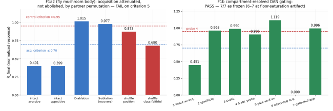
Figure 24: The F1 series under frozen criteria. Left: F1a2 run-mean R_{\text{final}} by arm — acquisition intact (blue), abolition controls (red): partner permutation attenuates but does not abolish acquisition, failing the > 0.95 abolition criterion under both readings (0.873 position-based; 0.680 class-faithful). Right: F1b compartment-resolved DAN gating — all seven frozen criteria MET as frozen (green; criteria 6–7 met at a floor-saturation value that is a calibration artifact, so the evidential weight rests on criteria 1–5). Per-run values and curves: simfl_work deposit (OSF, DOI: [insert]).
