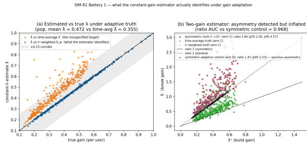
Figure SR4. SIM-R1 battery 1: (a) \hat{\lambda} versus the time-average \bar{\lambda} and versus the \varepsilon^2 -weighted \bar{\lambda}_w with the \pm 0.15 corridor; population mean \hat{\lambda} = 0.472 versus \bar{\lambda} = 0.355 — inside the H2 corridor while the truth lies outside. (b) Two-gain scatter: asymmetric truth \lambda^- = 2\lambda^+ (recovered ratio 2.84; weighted-truth ratio 2.845) versus the symmetric-adaptive control (spurious ratio mean 1.41, p95 2.23); direction AUC 0.968 (§6).
