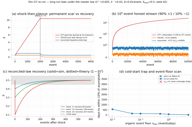
Figure S6. Sim G7: long-run dynamics of the three master-law presets ( \lambda^+ = 0.005 , \lambda^- = 0.02 , \delta = 0.01/\text{event} , S_{base} = 0.5 ). Shock-then-silence, 10^5 -event horizons, recovery curves (69/138/207 events to within 10% of baseline after -5/-10/-20 shocks under the baseline-restoring preset), and the cold-start scan (§3.2, §3.6).
