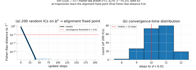
Figure S2. Sim G1(a): convergence to the alignment fixed point from 200 random initial conditions on \Delta^4 (planted \lambda = 0.35 ). Fisher–Rao distance trajectories and convergence-time histogram: final distance 0.0 for all trajectories, median 10 steps to d < 0.01 (§3.6).
