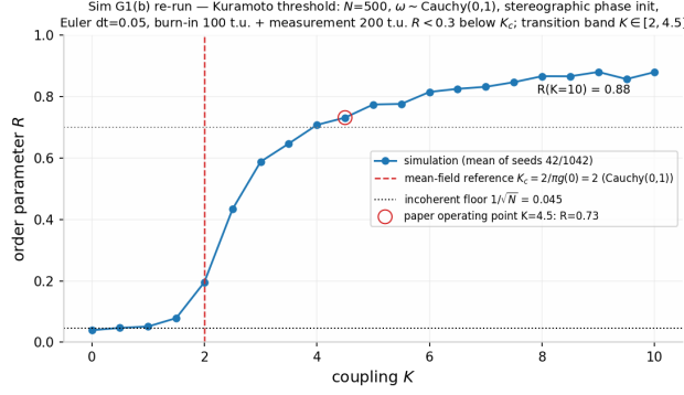
Figure S3. Sim G1(b): Kuramoto order parameter R versus coupling K ( N = 500 , unit-Cauchy natural frequencies). Incoherent ( R < 0.3 ) everywhere below the mean-field reference K_c = 2 (Eq. (21)); finite-size floor 1/\sqrt{N} ; PAS-level coherence ( R > 0.7 ) by K \approx 4.5 . Analogy structure only (§3.4, §3.6).
