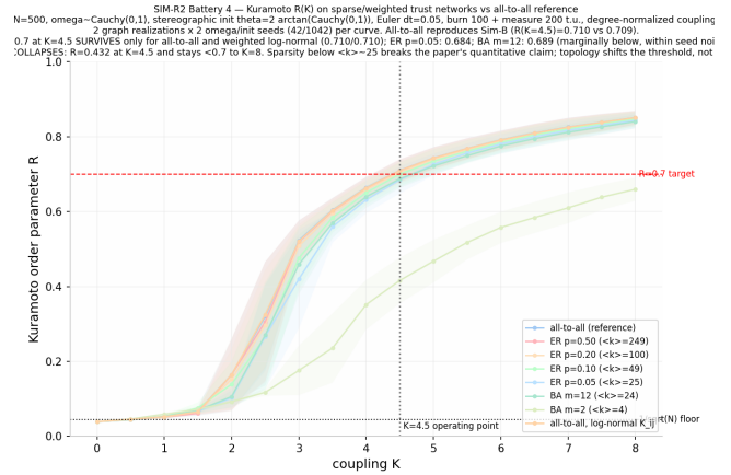
Figure SR2. SIM-R2 battery 4: Kuramoto R(K) per topology (mean \pm sd over 2 graph realizations \times 2 seeds) against the all-to-all reference, with the R = 0.7 target, the 1/\sqrt{N} floor, and the K = 4.5 operating point marked. The onset K_c \approx 2 is topology-invariant; the K = 4.5 coherence level is not (§3.4).
