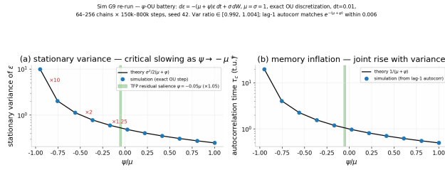
Figure S8. Sim G9: \psi battery. Stationary variance and autocorrelation time versus \psi/\mu with theory curves \sigma^2/(2(\mu + \psi)) and 1/(\mu + \psi) ; simulated/theory variance ratio within [0.992, 1.004] ; the dissipation-floor-slowness asymptote as \psi \rightarrow -\mu^+ (§3.3, §3.6).
