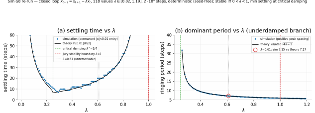
Figure S7. Sim G8: closed-loop \lambda battery. Settling time and dominant ringing period versus \lambda : asymptotic stability iff 0 < \lambda < 1 ; critical damping at \lambda^* = 1/4 , with the settling minimum on the plateau \lambda \in [0.25, 0.29] ; ringing period 7.15 simulated versus 7.17 predicted at \lambda = 0.61 (§3.6).
