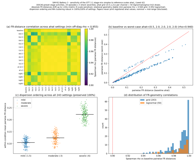
Figure SR1. SIM-R2 battery 3 ( \hat{a}_i sensitivity of the §3.1 Fisher–Rao simplex): (a) 21-setting Spearman- \rho heatmap of pairwise FR distances against the baseline; (b) baseline versus worst-case pairwise distances; (c) per-condition dispersion across all 243 grid settings — the mild < moderate < severe ordering never inverts; (d) \rho distributions (grid and log-normal perturbations).
