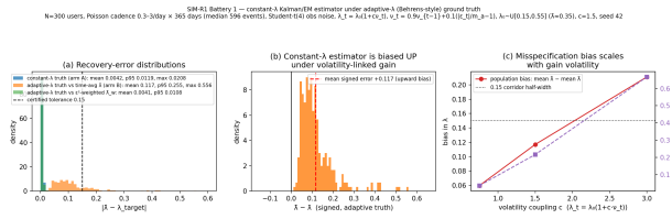
Figure SR3. SIM-R1 battery 1 ( N = 300 , seed 42): (a) |\hat{\lambda} - \lambda_{\text{target}}| under constant truth (mean 0.0042), adaptive truth against the time-average \bar{\lambda} (mean 0.117; 21.7% outside the 0.15 corridor), and adaptive truth against the \varepsilon^2 -weighted \bar{\lambda}_w (mean 0.0041); (b) signed error showing the +0.117 upward bias; (c) population bias and corridor-breach fraction versus volatility coupling c \in \{0.75, 1.5, 3.0\} (§6).
