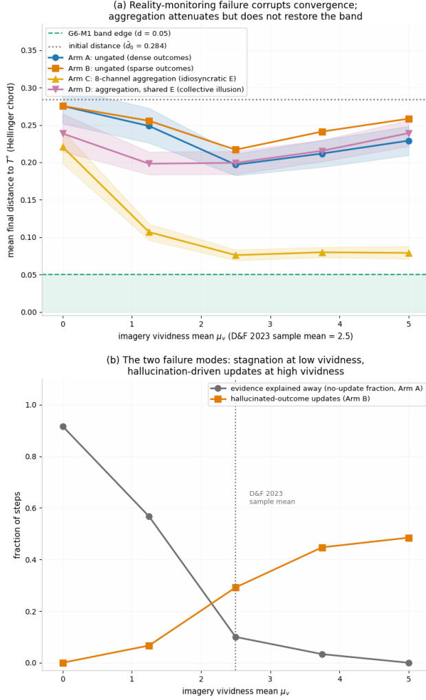
Figure SR6. Reality-monitoring corruption of trust-stage dynamics (Sim G22, seed 20260913; pre-registered frozen criteria). (a) Mean final distance to the true target T^* across the imagery-vividness grid: ungated observers (dense and sparse outcome regimes) sit far outside the G6-M1 convergence band (green) at and above the source study’s sample mean (2.5); eight-channel aggregation attenuates the bias \approx 2.9\times but does not restore the band, and fails entirely when expectations are shared (collective-illusion arm). Shaded ribbons: 95% bootstrap CIs. (b) The two failure modes: evidence explained away (stagnation) at low vividness; hallucinated-outcome updates under sparse outcomes at high vividness. Verdicts per frozen criteria: C1–C4, C6 PASS; C5 FAIL; compound FAIL. Pre-registration, closure note, code, and results JSON in the deposit.
