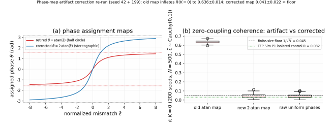
Figure S1. Phase-map control battery (200 seeds, K = 0 , N = 500 , Cauchy(0,1) mismatches; §3.4). (a) The half-circle arctan map occupies only half the circle; the stereographic map \theta = 2 \arctan(\tilde{\varepsilon}) covers it. (b) Zero-coupling coherence: the half-circle map reports R = 0.636 \pm 0.014 (artifact); the stereographic map restores the finite-size floor at 0.041 \pm 0.022 , matching raw uniform phases ( 0.042 \pm 0.021 ) and the TFP Sim P1 isolated control ( R = 0.032 ).
