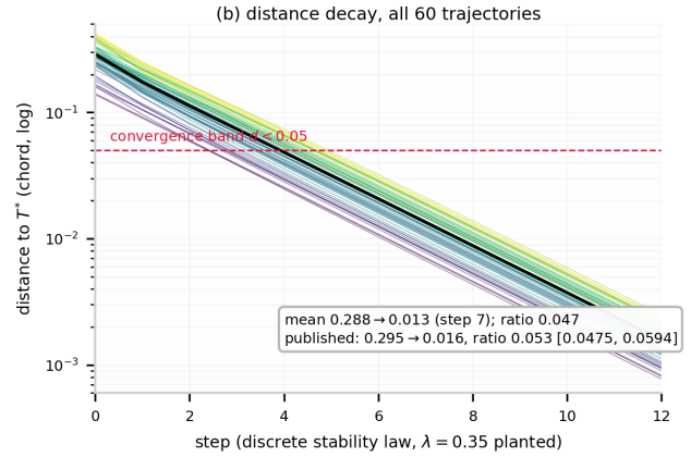
Figure SR5. The trust manifold rendered (Sim G6-M1, independent re-implementation of the published specification; seed 20260908). (a) 3-D PCA embedding of the centered simplex \Delta^4 (81.8% of trajectory variance): 60 stage-mix trajectories (light \rightarrow dark with time; orange markers: initial conditions; red arrows: flow direction) contract radially onto the alignment attractor T^* (gold star) — exactly radial under the linear law, uniform contraction made visible; the faint wireframe is the projected simplex frame. (b) Distance decay (Hellinger chord, the convention of the printed G6-M1 values): every trajectory enters the d < 0.05 convergence band. Interactive version, code, and results JSON in the deposit (figures/gtt/, sim-code/, numbers/).
