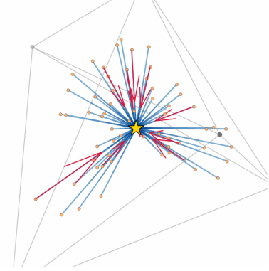
(a) 3-D PCA embedding of the centered simplex \Delta^4 (81.8% of variance): radial contraction onto T^*
