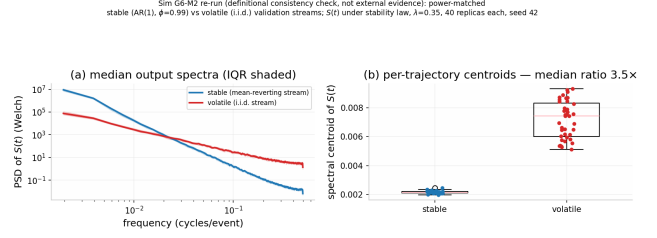
Figure S4. Sim G6, M2 (definitional consistency check): median output power spectra of S(t) and per-trajectory spectral centroids for stable versus volatile validation streams (40 replicas per condition, post-transient Welch spectra). Median centroid ratio 3.5\times , BCa 95% CI [3.04, 3.69]; complete separation (Mann–Whitney p = 7.2 \times 10^{-15} ). A check that the stable/volatile definition is operational, not external evidence (§3.6).
