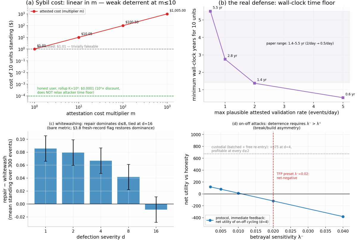
Figure 9: Sim P8 (§3.7), explicit master-law preset \lambda^- = 0.02 , \lambda^+ = 0.005 , \delta = 0.01/\text{event} : (a) Sybil cost versus attestation multiplier m (log-log; $1.01 unattested \rightarrow $1,005 at m = 1,000 for 10 units of standing) with the block-rollup honest-cost baseline ( 10^{-7}/\text{event} at K = 10^4 events per anchor); (b) the wall-clock time floor quoted per rate (5.5/1.4 years for 1,005 attested events at 0.5/\leq 2 events/day; \sim 0.55\text{--}1.1 years at the model’s own high-standing rates of 2.5\text{--}3.76 events/day, 5/day max grid; 0.73 yr at 3.76/day; 0.55 yr at 5/day; parallel-provider collusion divides the floor, §3.7); (c) repair-versus-whitewash standing advantage by defection severity — significant for d \leq 8 , statistically tied at d = 16 under the bare standing metric; (d) on-off cycling net utility versus \lambda^- : net-negative exactly at the \lambda^- = 0.02 preset under immediate feedback, while custodial batched feedback with free re-entry stays profitable at every d \geq 2 .
