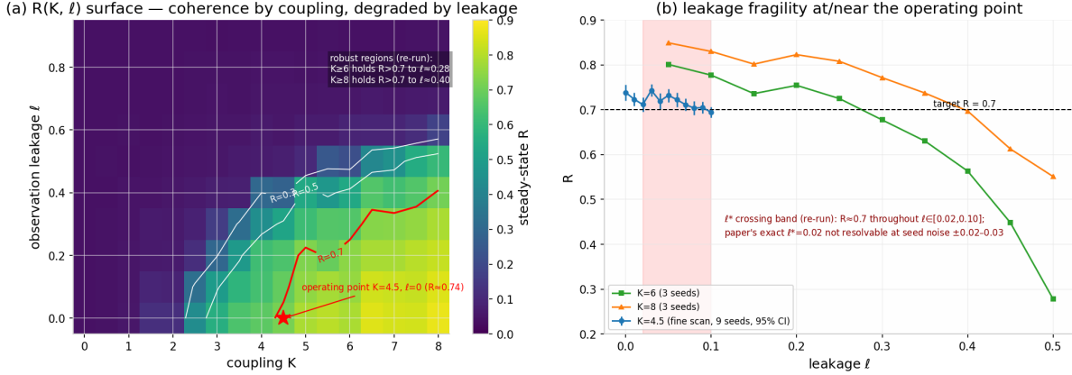
Figure 7: Sim P1b (§3.6): the coherence surface R(K, \ell) over K \in [0, 8] \times \ell \in [0, 0.9] with R = 0.3/0.5/0.7 contours and the K = 4.5 operating point marked, and the leakage-fragility slice with the crossing band \ell^* \in [0.02, 0.10] (9-seed fine scan). Leakage model: K_{\text{eff}} = K(1 - \ell) plus observation noise \sigma_\eta = \pi\ell/2 redrawn every timestep; N = 500 , \omega \sim \text{Cauchy}(0, 1) , stereographic initialization, dt = 0.05 . Robust regions (two independent seeded re-renders; point precision not resolvable at these N ): K = 6 holds R > 0.7 to \ell \approx 0.22-0.28 ; K = 8 to \ell \approx 0.30-0.40 ; the R = 0.7 contour sits at K \approx 5.0-5.5 ( \ell = 0.1 ) and K \approx 5.9-7 ( \ell = 0.2 ), retreating off-grid ( K > 8 ) only for \ell \gtrsim 0.25-0.4 across re-renders; \ell is a model-internal parameter with no field operationalization yet.
