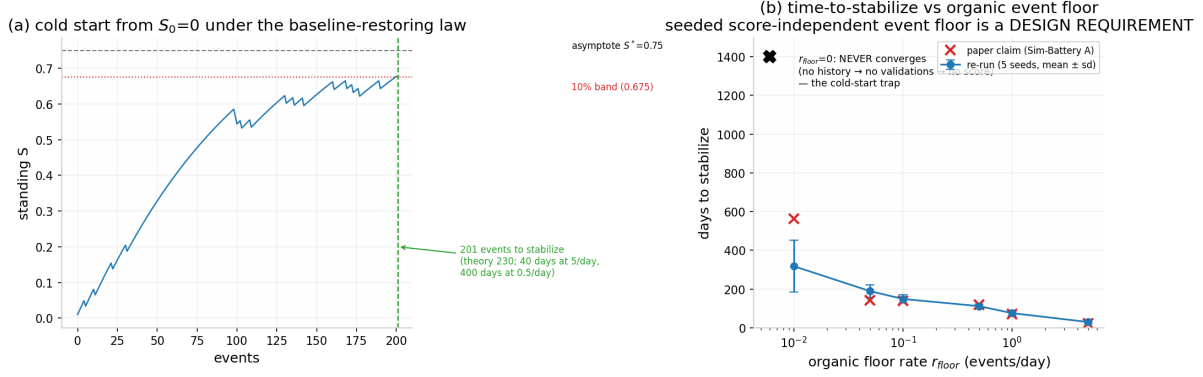
Figure 13: Cold start and the event floor (§3.10; baseline-restoring law, \lambda^+ = 0.005 , \lambda^- = 0.02 , \delta = 0.01/\text{event} , S_{\text{base}} = 0.5 ): from S_0 = 0 the law stabilizes within 10% of the asymptote in 201 events; with rate feedback r = r_{\text{floor}} + 5S/\text{day} , r_{\text{floor}} = 0 never converges (the trap, exact), and escape times run 318 \pm 133 days at r_{\text{floor}} = 0.01/\text{day} down to 30 days at 5/day under the first-crossing criterion ( S \geq 0.9 S^* , S^* = 0.75 ; 189/149/112/76 days at 0.05/0.1/0.5/1 per day), with stabilization-to-asymptote at days 563/144/140/120/72/24 across the same floor grid — both criteria verified; the earlier single-grid printing conflated them.
