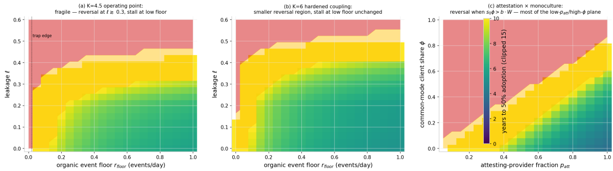
Figure 14: Adoption-compounding sensitivity (§3.10(iii)), toy densification-feedback model of Eq. (6) with labeled assumptions: outcome maps over the (r_{\text{floor}}, \ell) plane at K = 4.5 (39% compound / 28% stall / 33% reversal) and K = 6 (54%/26%/20%), and over the (p_{\text{att}}, \phi) plane ( K = 6 , \ell = 0.05 , r_{\text{floor}} = 0.5 ). Compounding requires r_{\text{floor}} \gtrsim 0.15/\text{day} even at \ell = 0 , p_{\text{att}} \gtrsim 0.6 at \phi = 0.2 , or \phi \lesssim 0.42 at p_{\text{att}} = 0.8 .
