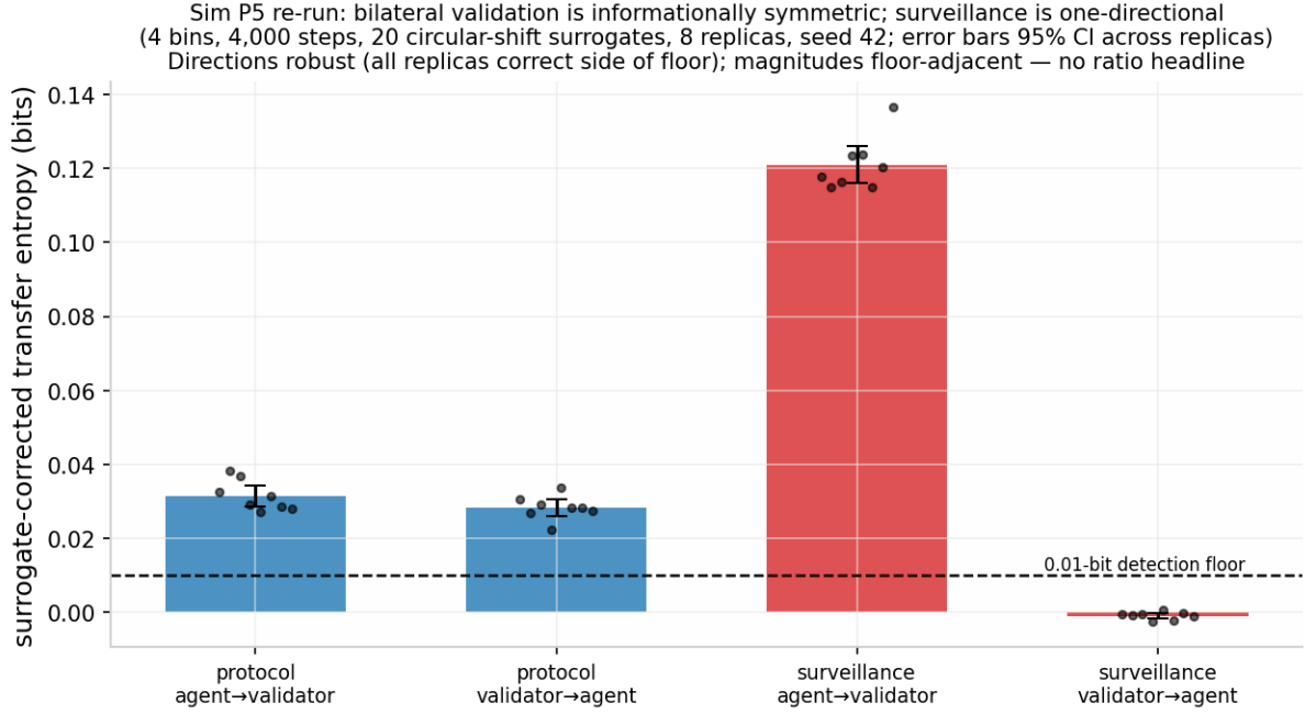
Figure 10: Sim P5 (§3.7): surrogate-corrected transfer entropy between agent and validator under bilateral validation (protocol: 0.0315 \pm 0.003 / 0.0283 \pm 0.002 bits) versus surveillance ( 0.121 \pm 0.005 / -0.001 \pm 0.001 bits), 95% CIs across 8 replicas, with the 0.01-bit detection floor marked; every replica lands on the correct side of the floor in both architectures. Magnitudes are floor-adjacent, so no ratio headline is reported.
