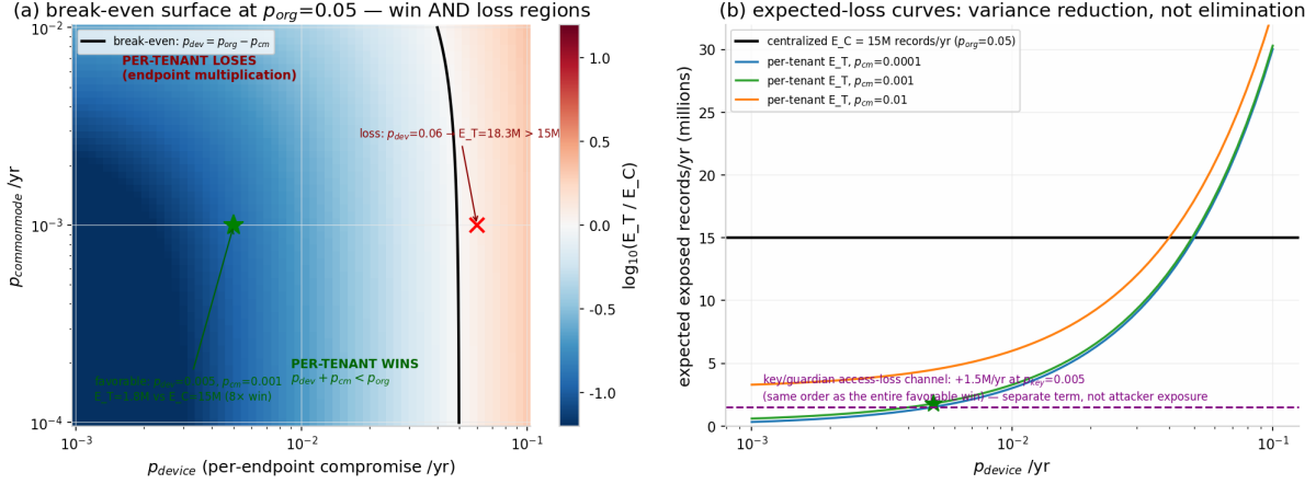
Figure 12: Expected-loss threat model (§3.9), N_{all} = n_{devices} = 3 \times 10^8 : (a) \log_{10}(E_T/E_C) over p_{device} \times p_{commonmode} at p_{org} = 0.05 with the break-even contour p_{device} = p_{org} - p_{commonmode} ; (b) expected-loss curves — centralized 15M records/yr at p_{org} = 0.05 ; per-tenant 1.8M/yr in the favorable region ( p_{device} = 0.005 , p_{cm} = 0.001 ) and 18.3M/yr at p_{device} = 0.06 — with the key/guardian access-loss term (+1.5M/yr at p_{key} = 0.005 ) shown separately. Variance reduction, not elimination.
