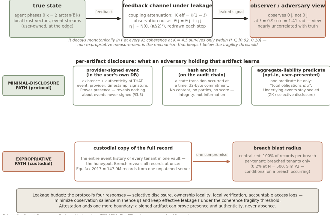
Figure 6: The observation-leakage model (§3.6, Sim P1b; supports §3.8–3.9). Top: leakage \ell \in [0,1] degrades the feedback channel two compounding ways — coupling attenuation K_{\text{eff}} = K(1 - \ell) and observation noise \hat{\theta}_j = \theta_j + \eta_j , \eta_j \sim \mathcal{N}(0, (\pi\ell/2)^2) — so the adversary's view decorrelates from the true state as \ell rises (at \ell = 0.9 , \sigma_{\eta} \approx 1.41 rad). Middle: what each stored artifact reveals — a provider-signed event reveals that event's existence and authenticity only; a hash anchor reveals that a transition occurred, never content; an opt-in aggregate-liability predicate reveals one predicate bit (minimal-disclosure path) — versus the custodial path, where one compromise of the full-record vault exposes 100% of records (Equifax 2017 anchor; per-tenant conditional exposure 0.2% at N = 500 , Sim P2). Bottom: the leakage budget, model-internal: \ell has no field operationalization, and the mapping from the four responses (§4) (or from m/\psi ) to \ell is an unmeasured assumption; in the model, R > 0.7 at K = 4.5 requires \ell \lesssim 0.02\text{--}0.10 .
