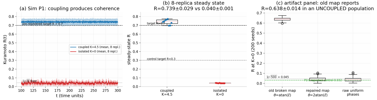
Figure 4: Sim P1 (§3.6): the Kuramoto order parameter R(t) under protocol coupling ( K = 4.5 ) versus the isolated control ( K = 0 ) across 8 replicas, with steady-state distributions (coupled R = 0.739 \pm 0.029 ; isolated R = 0.040 \pm 0.001 , at the 1/\sqrt{N} \approx 0.045 finite-size floor) and the phase-map-control side panel: the half-circle \text{atan} initialization reports R = 0.638 \pm 0.014 at K = 0 (200 seeds), while the corrected stereographic map ( 0.040 \pm 0.020 ) and raw uniform phases ( 0.039 \pm 0.020 ) sit at the floor. Verification re-run, seed 42.
