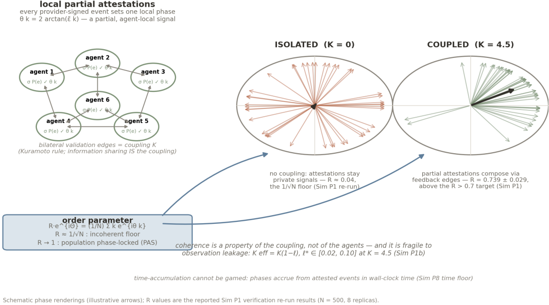
Figure 5: Partial attestations compose into coherence (§3.6, Sim P1; schematic). Each provider-signed event fixes one agent-local phase \theta_k = 2 \arctan(\tilde{e}_k) ; bilateral validation edges are the Kuramoto coupling K ; the order parameter R \cdot e^{i\Theta} = (1/N) \sum_k e^{i\theta_k} measures population alignment. Schematic phase renderings: isolated agents ( K = 0 ) sit at the 1/\sqrt{N} incoherent floor ( R \approx 0.04 ); the coupled population ( K = 4.5 ) phase-locks ( R = 0.739 \pm 0.029 , Sim P1 verification re-run). Coherence is a property of the coupling, not of the agents, and is fragile to leakage ( K_{\text{eff}} = K(1 - \ell) ; the \ell^* band at the operating point, Sim P1b); phases accrue from attested events in wall-clock time (the Sim P8 time floor), so accumulation cannot be compressed except by parallel-provider collusion (§3.7 caveat). Phase arrows are seeded schematic draws; only the printed re-run values are measured.
