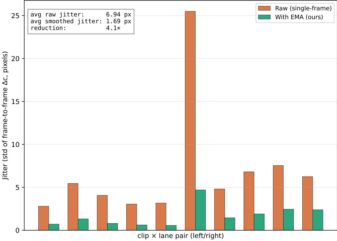
(C) Temporal Smoothing reduces jitter (4.1× average reduction)
