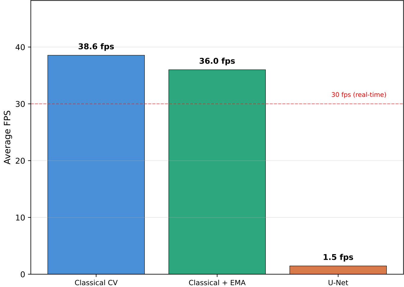
(B) Throughput on CPU (100 frames)
