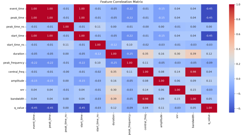
Figure 3.5: Pearson correlation between the twelve numerical Omicron descriptors. The three timestamps are perfectly correlated, and central frequency and bandwidth correlate at 0.98.
