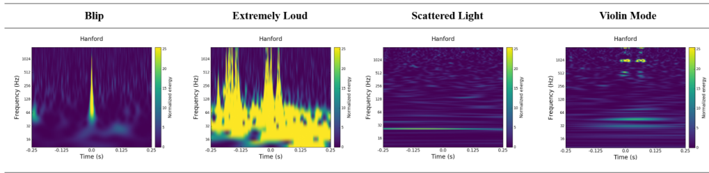
Figure 3.2: One Omega-scan spectrogram per retained class (Hanford detector, 0.5 s window). From left: a short teardrop-shaped transient, a saturated broadband event, a long low-frequency band, and narrow lines near 500 Hz and 1 kHz.
