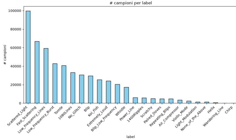
Figure 3.1: Class frequencies in the Gravity Spy machine-learning release, all observing runs and both detectors combined. The distribution is strongly imbalanced.
