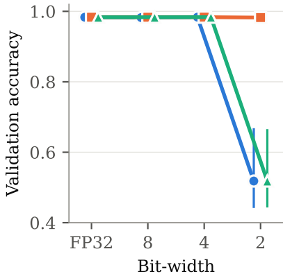
(a) Accuracy
