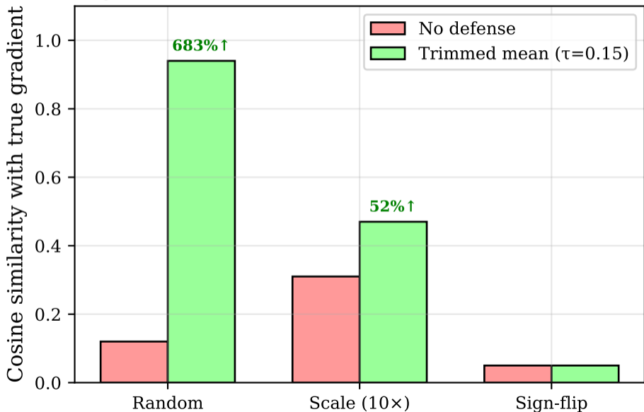
Byzantine Tolerance (20% adversarial workers)
