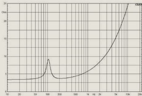
IMPEDANCE CURVE
