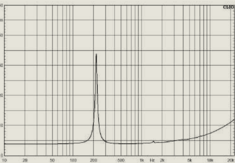
IMPEDANCE CURVE
