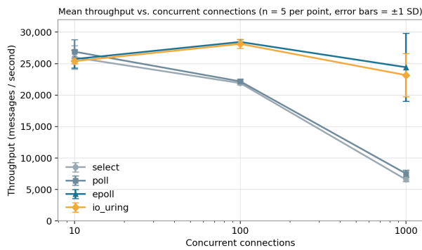
Figure 2: Mean throughput vs. connections ( n=5 , \pm 1 std. dev.).
