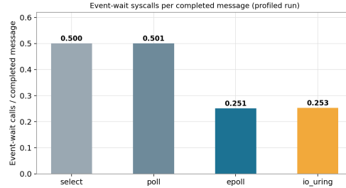
Figure 7: Event-wait calls per completed message (profiled run) — select/poll \approx 0.50, epoll/io_uring \approx 0.25.
