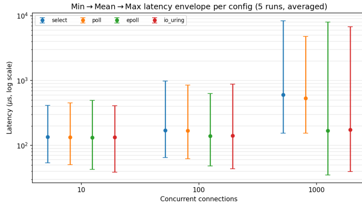
Figure 4: Min→mean→max latency envelope, averaged across the 5 core-benchmark runs per config (log scale). This is a real, measured spread — not a percentile plot: the underlying client stores only running min/mean/max per run, not individual per-request samples, so no p50/p90/p99 can be derived from it (see Fig. 5 for true percentiles from a separate measurement). True latency percentiles (supplementary pass). To close the percentile gap honestly rather than approximate it, we additionally ran each server at 1,000 connections under latency_profiler.py , an asyncio client that times every individual request/response round trip and sorts the resulting sample array. This is a genuinely different measurement (10 messages/connection, one repetition, same machine) from the core benchmark above, not a reprocessing of it.
