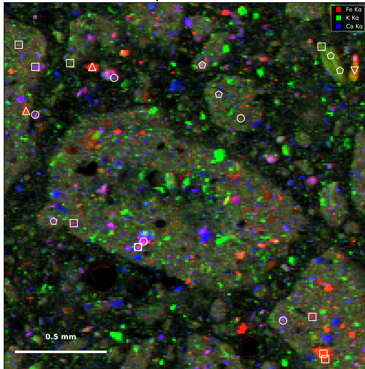
Map 12 — Fe/K/Ca
