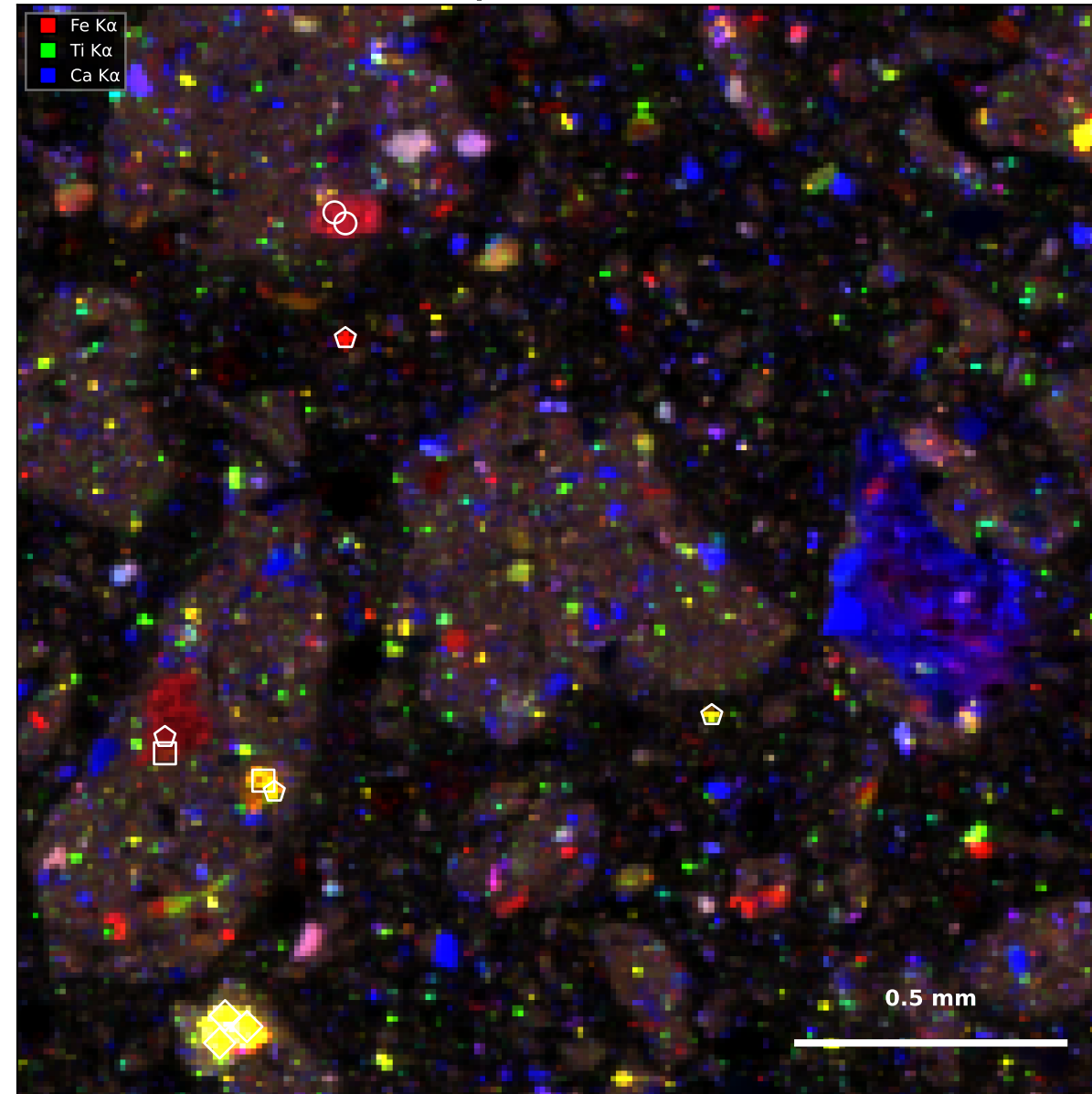
Map 5 — Fe/Ti/Ca
