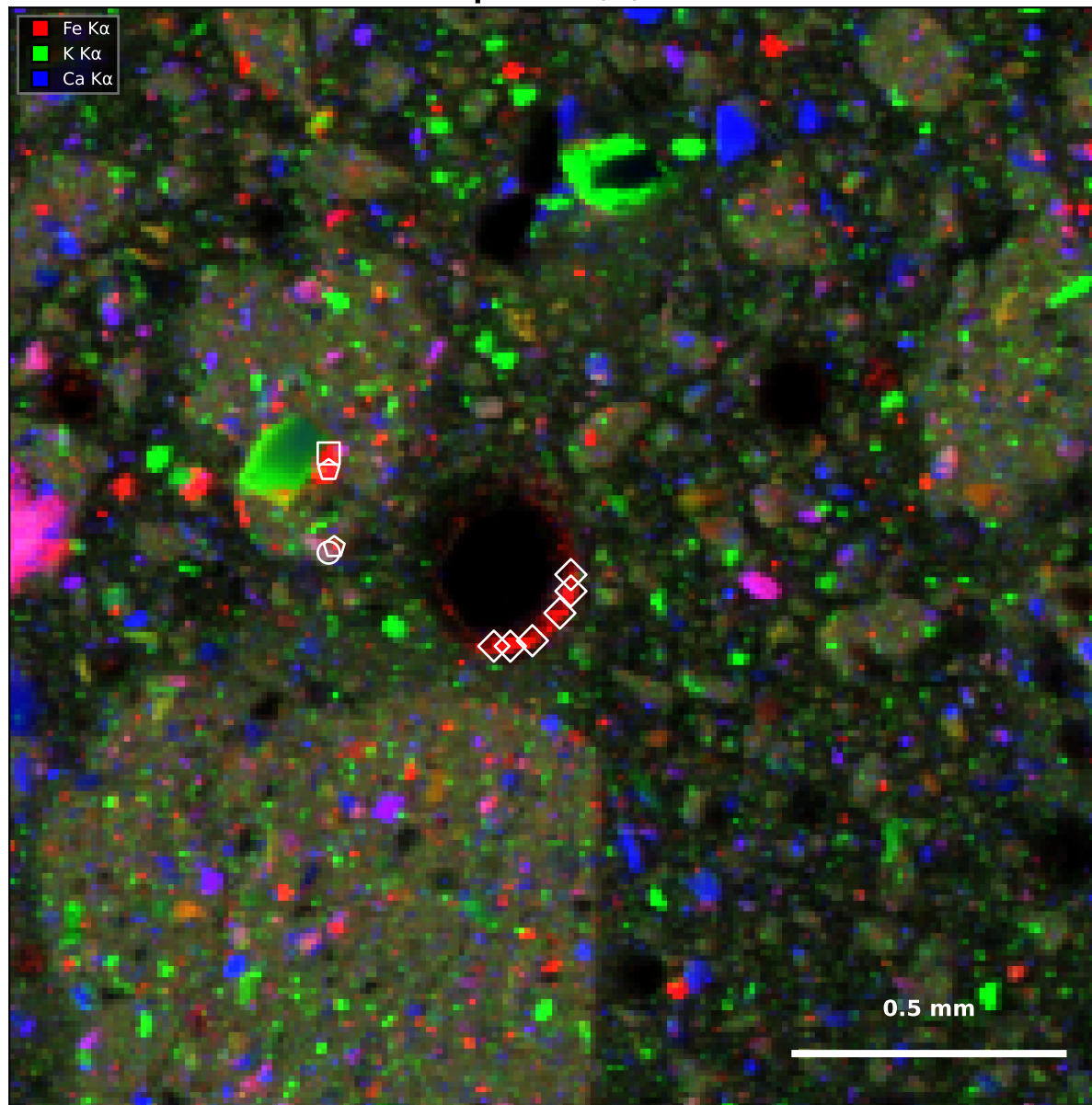
Map 8 — Fe/K/Ca
