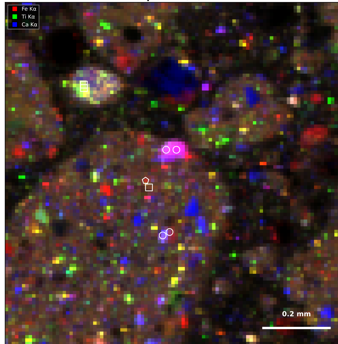
Map 2 — Fe/Ti/Ca
