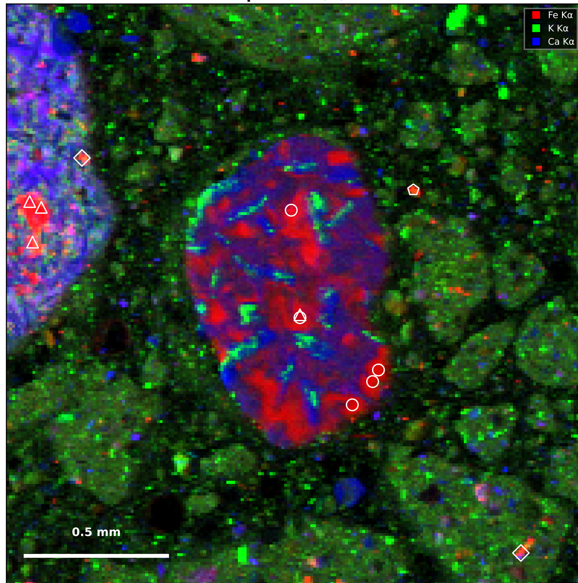
Map 10 — Fe/K/Ca
