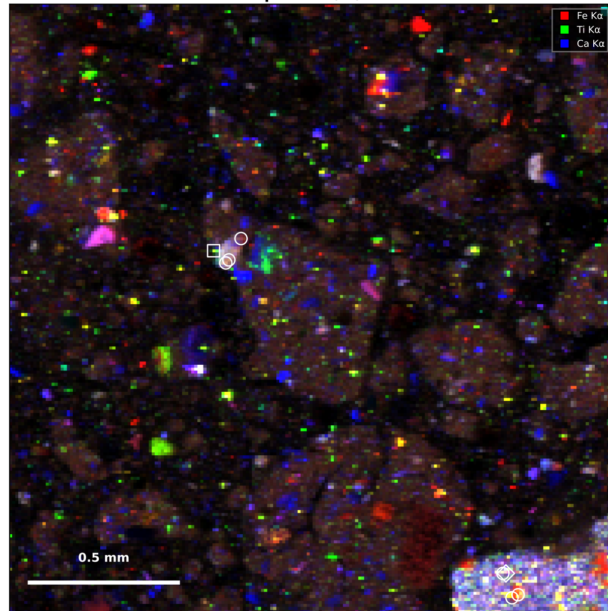
Map 4 — Fe/Ti/Ca
