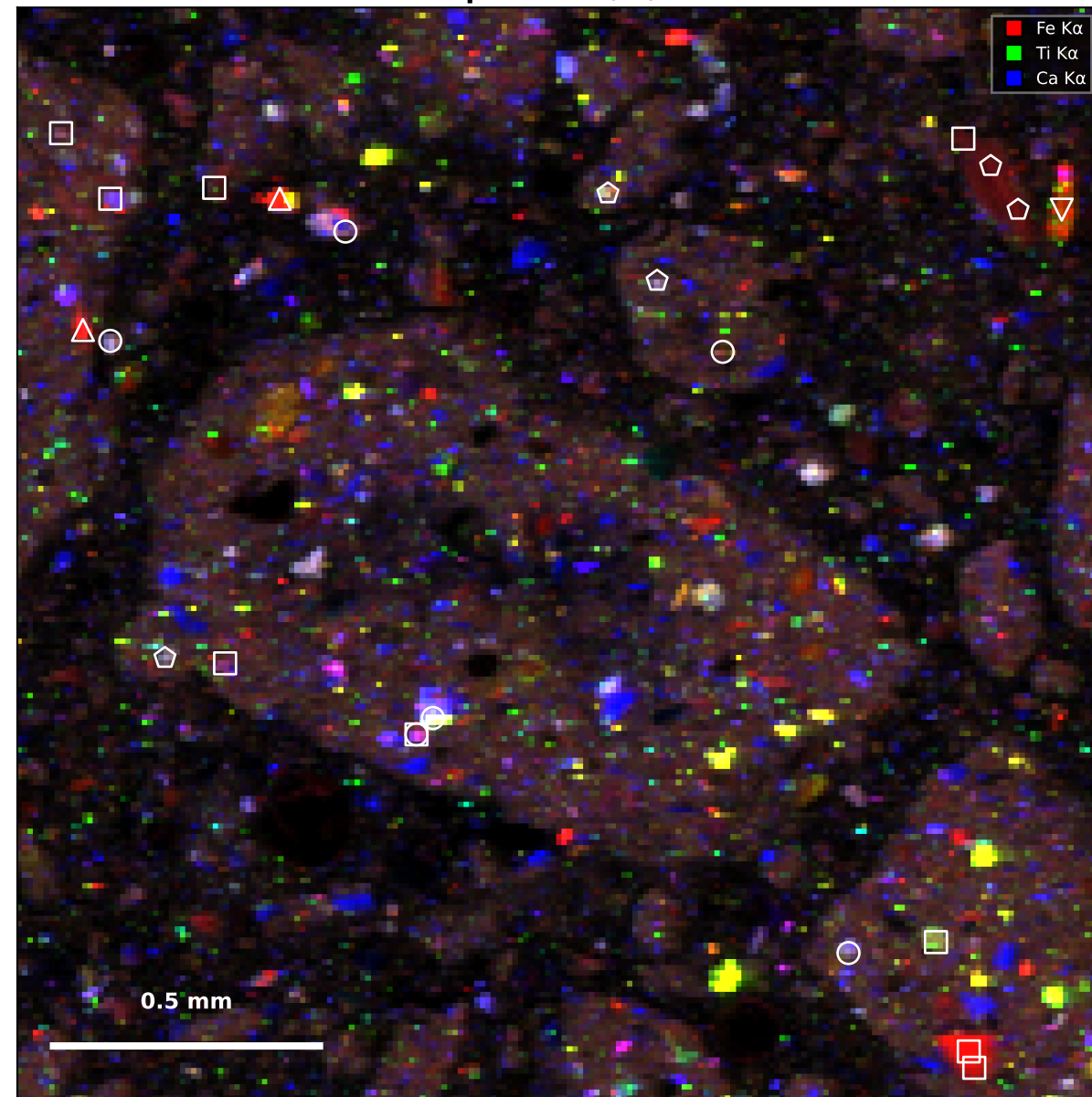
Map 12 — Fe/Ti/Ca
