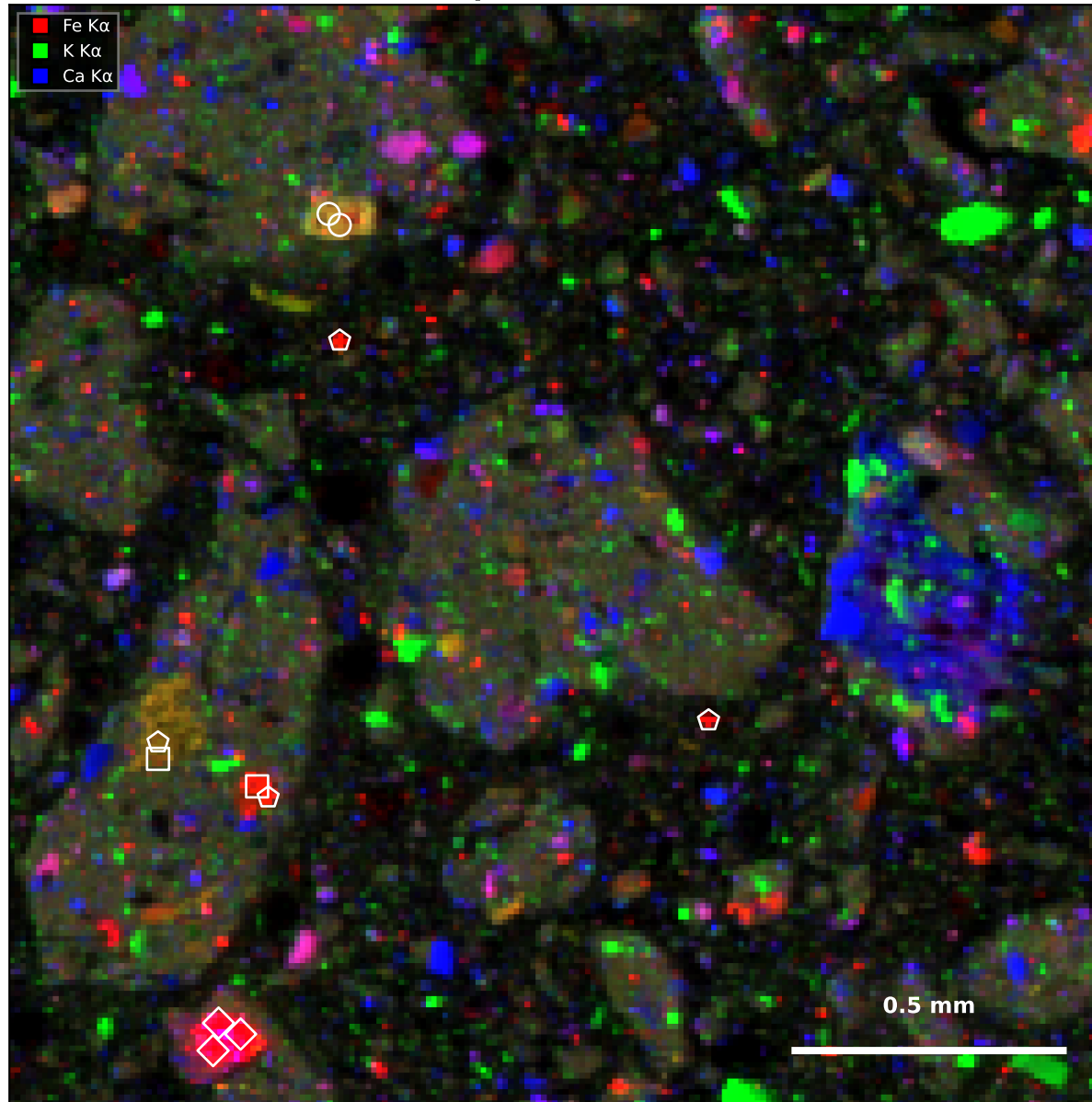
Map 5 — Fe/K/Ca
