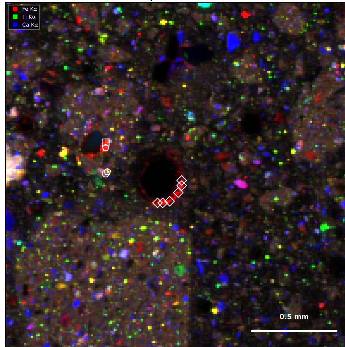
Map 8 — Fe/Ti/Ca
