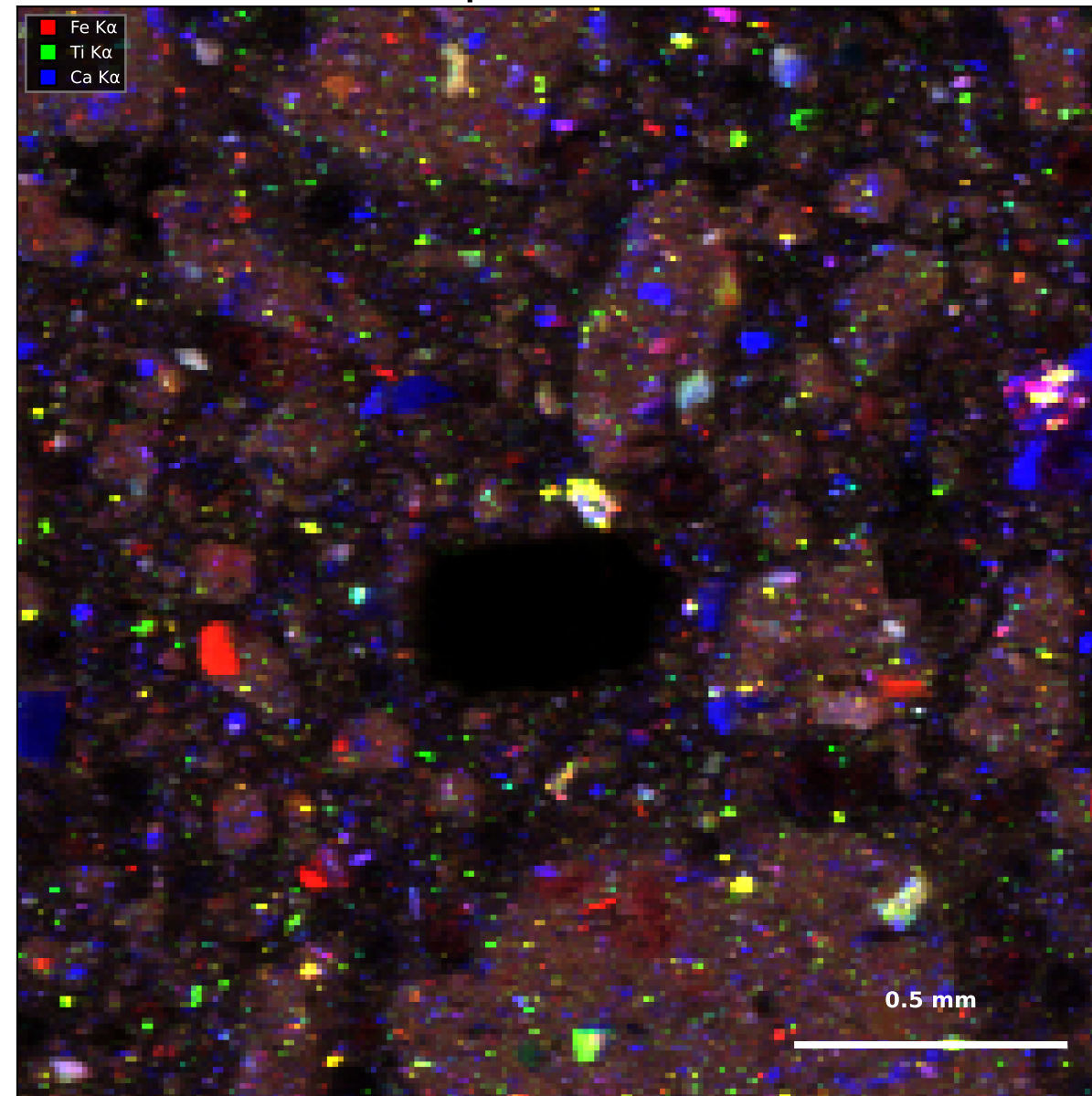
Map 13 — Fe/Ti/Ca
