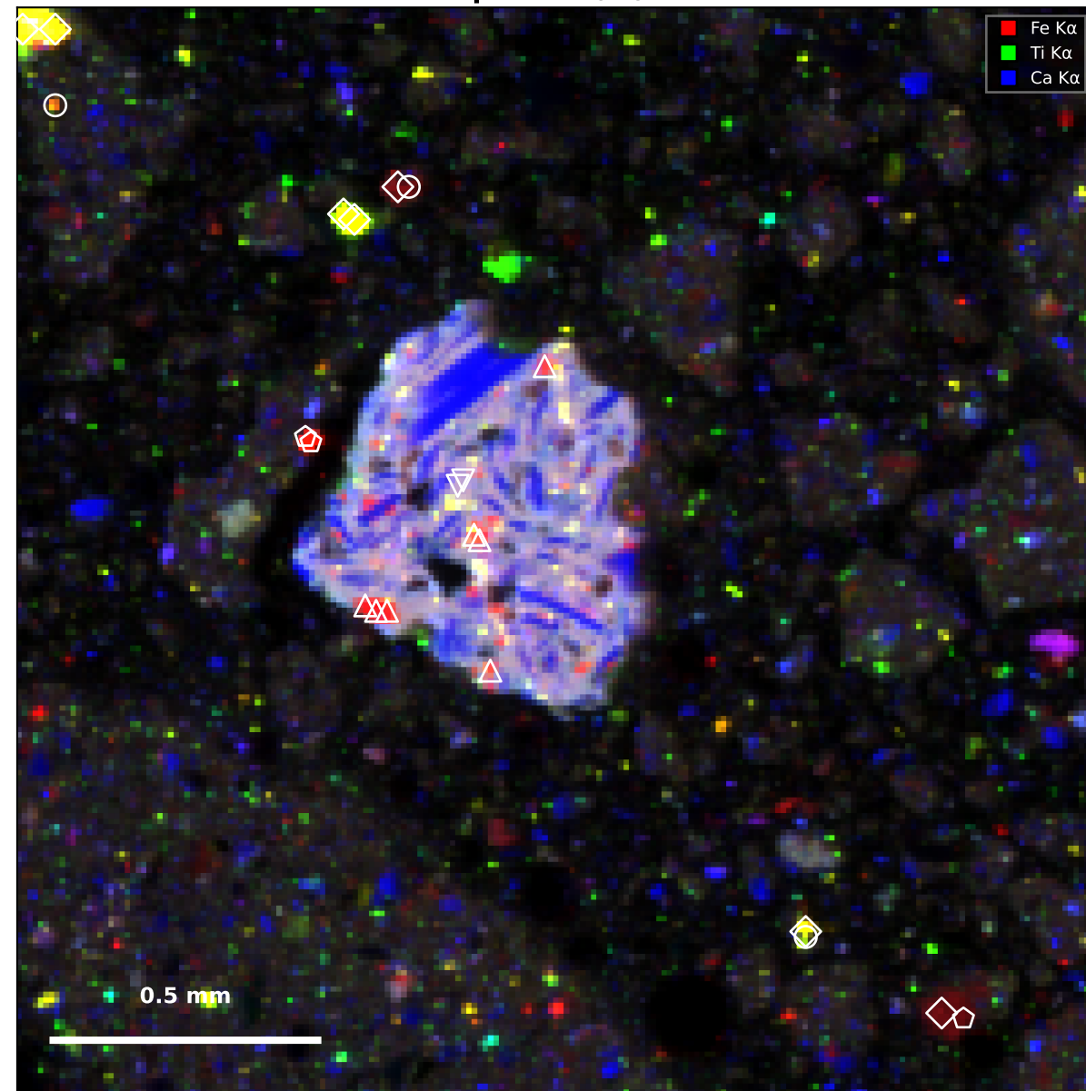
Map 9 — Fe/Ti/Ca
