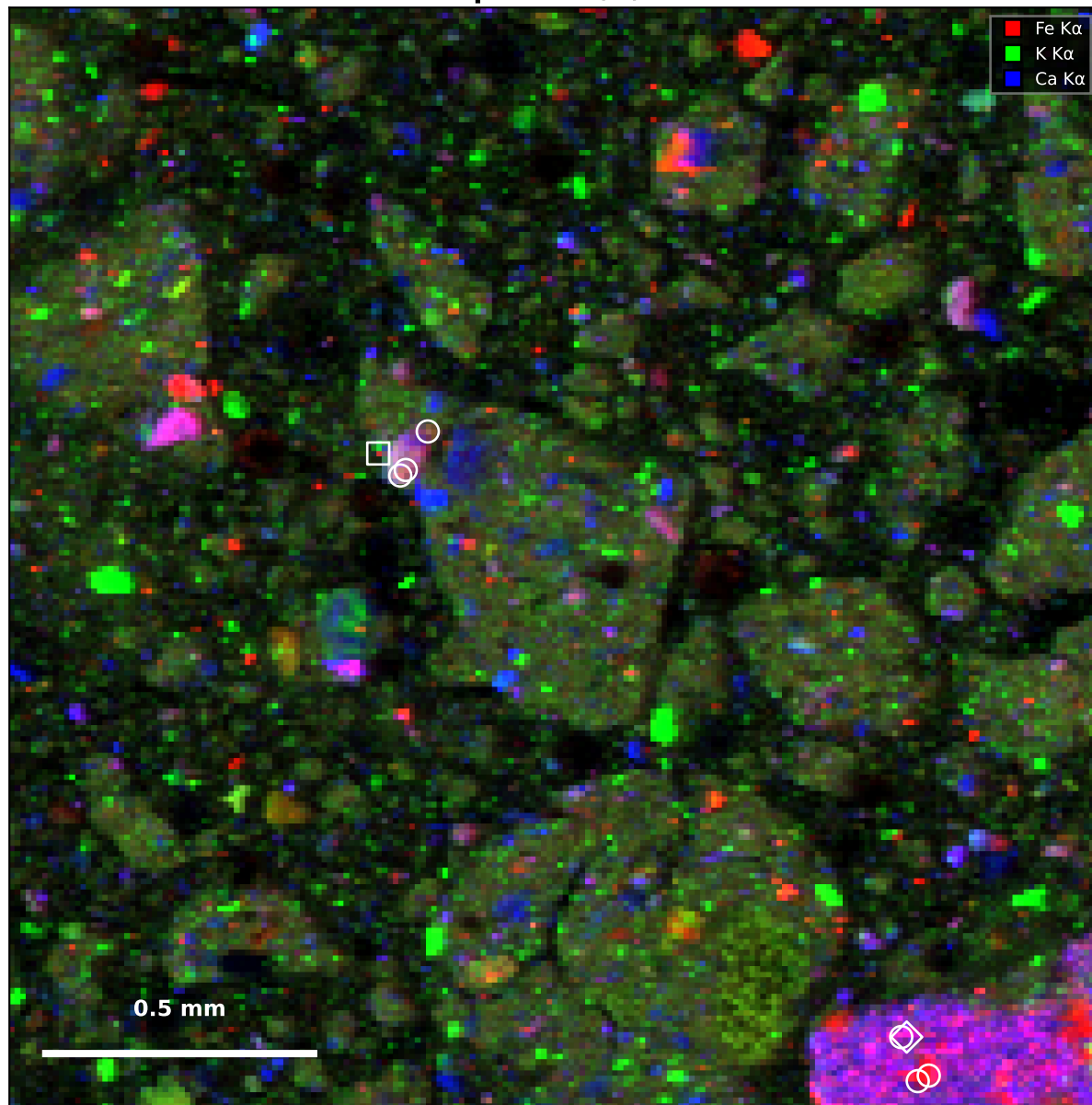
Map 4 — Fe/K/Ca
