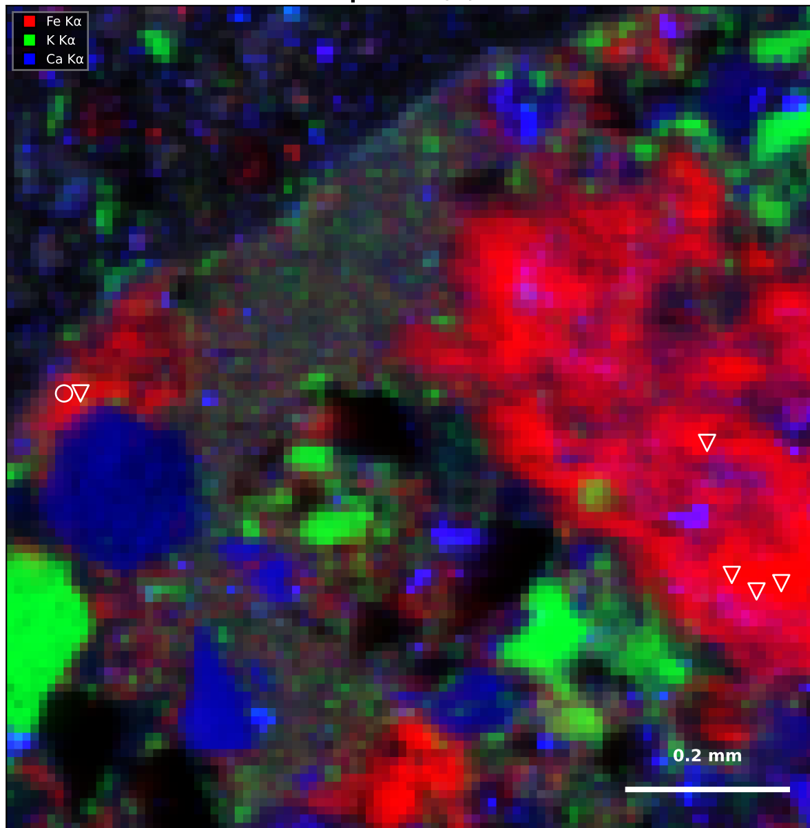
Map 1 — Fe/K/Ca
