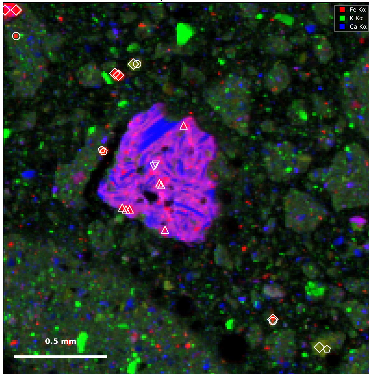
Map 9 — Fe/K/Ca
