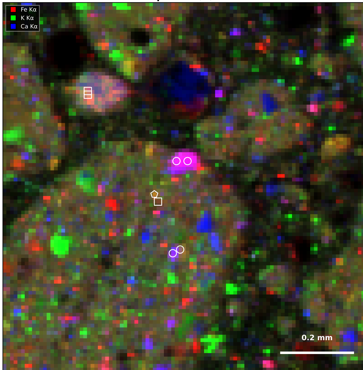
Map 2 — Fe/K/Ca
