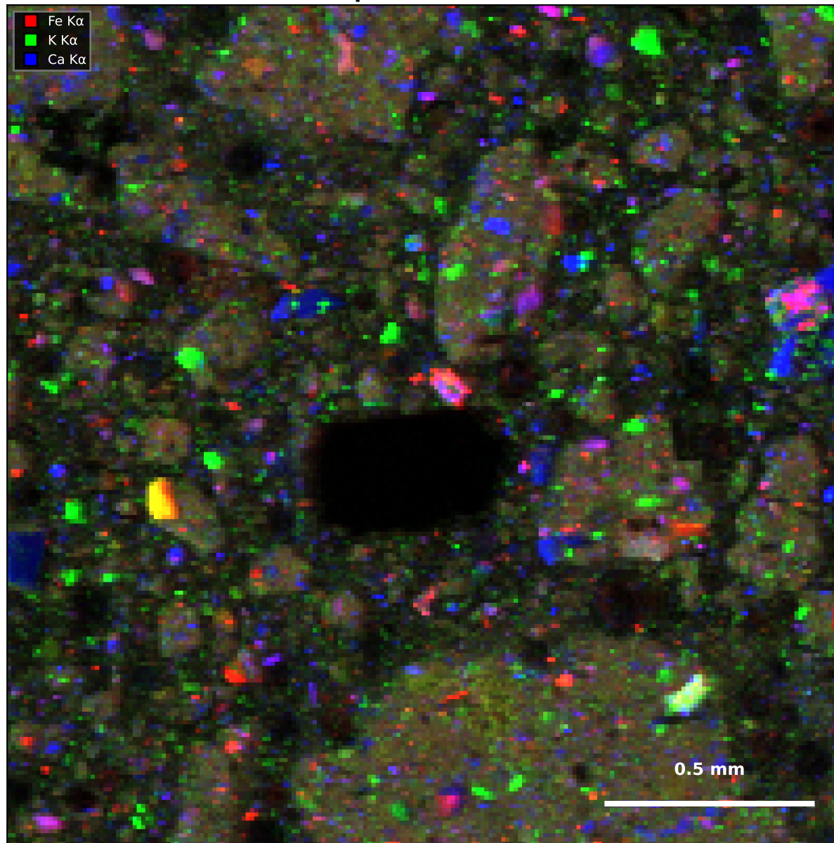
Map 13 — Fe/K/Ca
