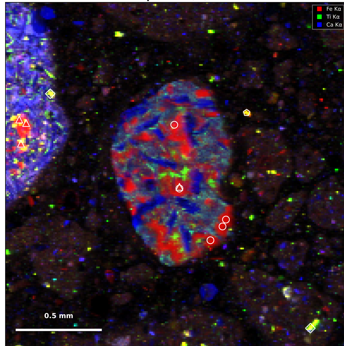
Map 10 — Fe/Ti/Ca
