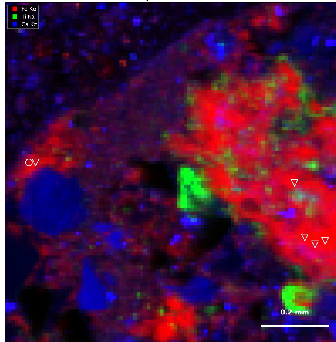
Map 1 — Fe/Ti/Ca
