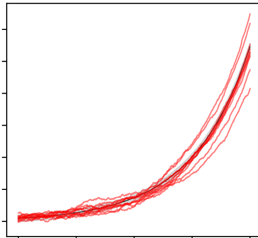
mean field ( N = 100 )
