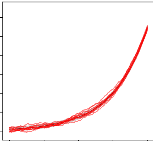
forward equivalent
