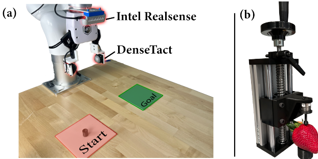
Fig. 3: On the left (a) is the experimental setup. The fruit is initially place in the starting zone on the black pedestal and then lifted to the green goal region. The two sensing modalities used are highlighted in red: the DenseTact optical tactile sensor and IntelRealsense D435i. On the right (b) is the force measuring apparatus which is used to quantify internal damage in the fruit.
