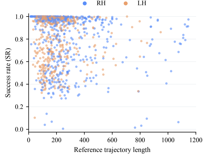
Fig. 2: Per-trajectory success rates versus reference trajectory length. Colors distinguish right-hand (RH) and left-hand (LH) trajectories.
