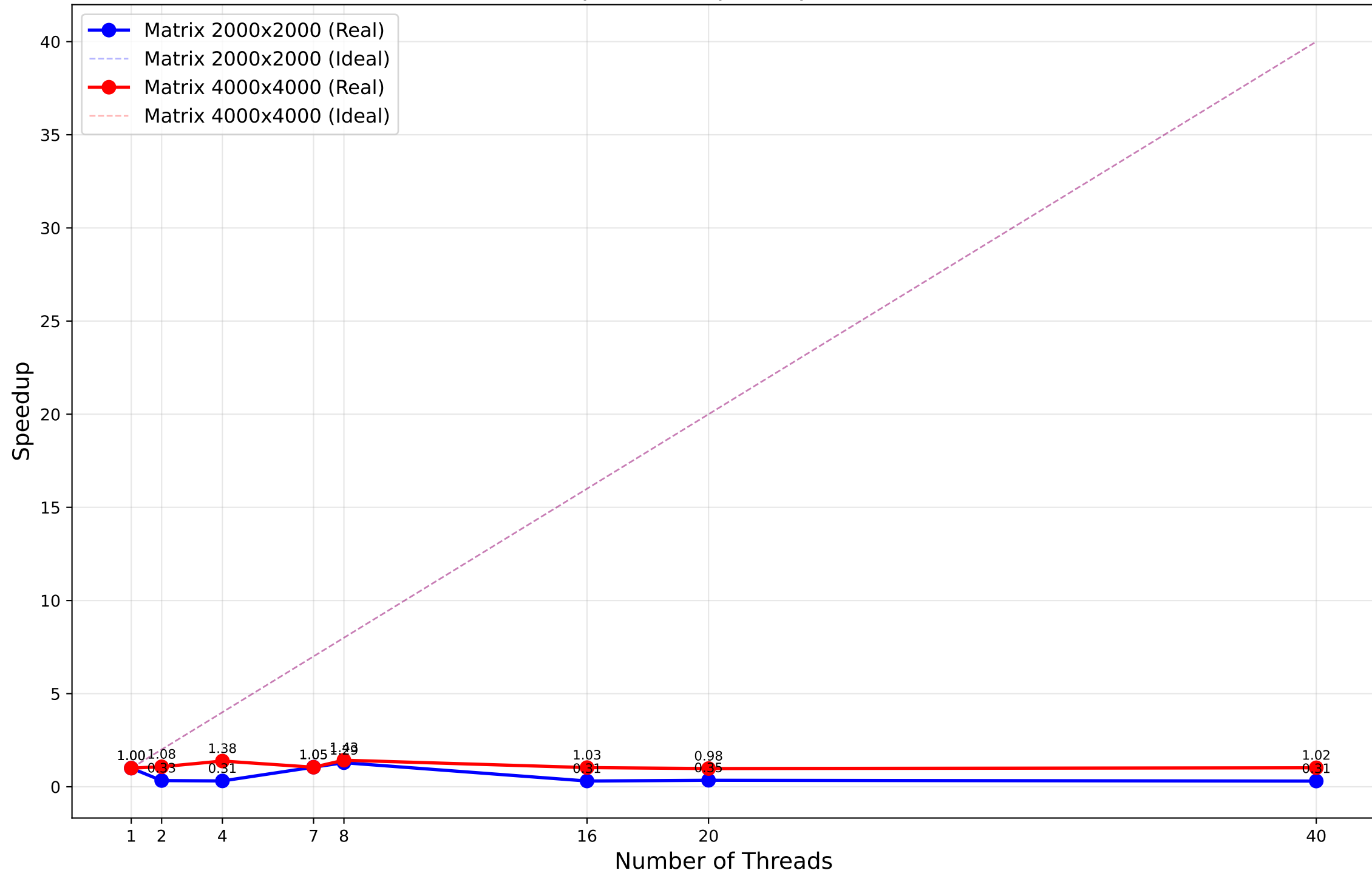
Matrix-Vector Multiplication Speedup vs Number of Threads
