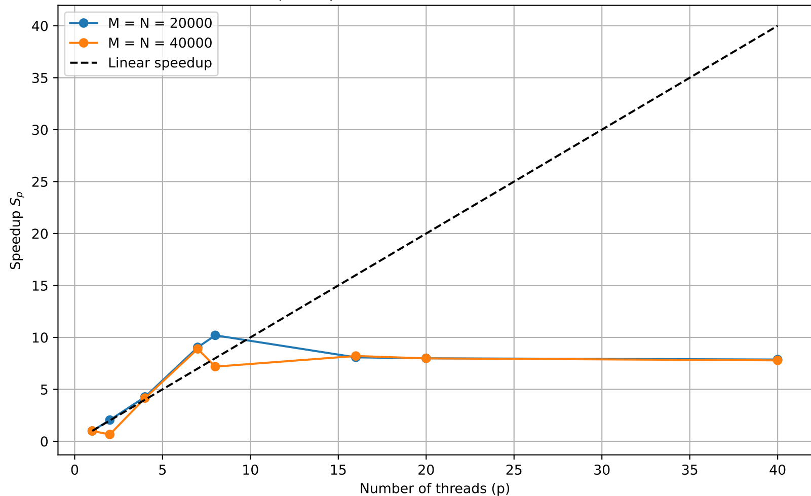
Speedup vs Number of Threads (DGEMV)
