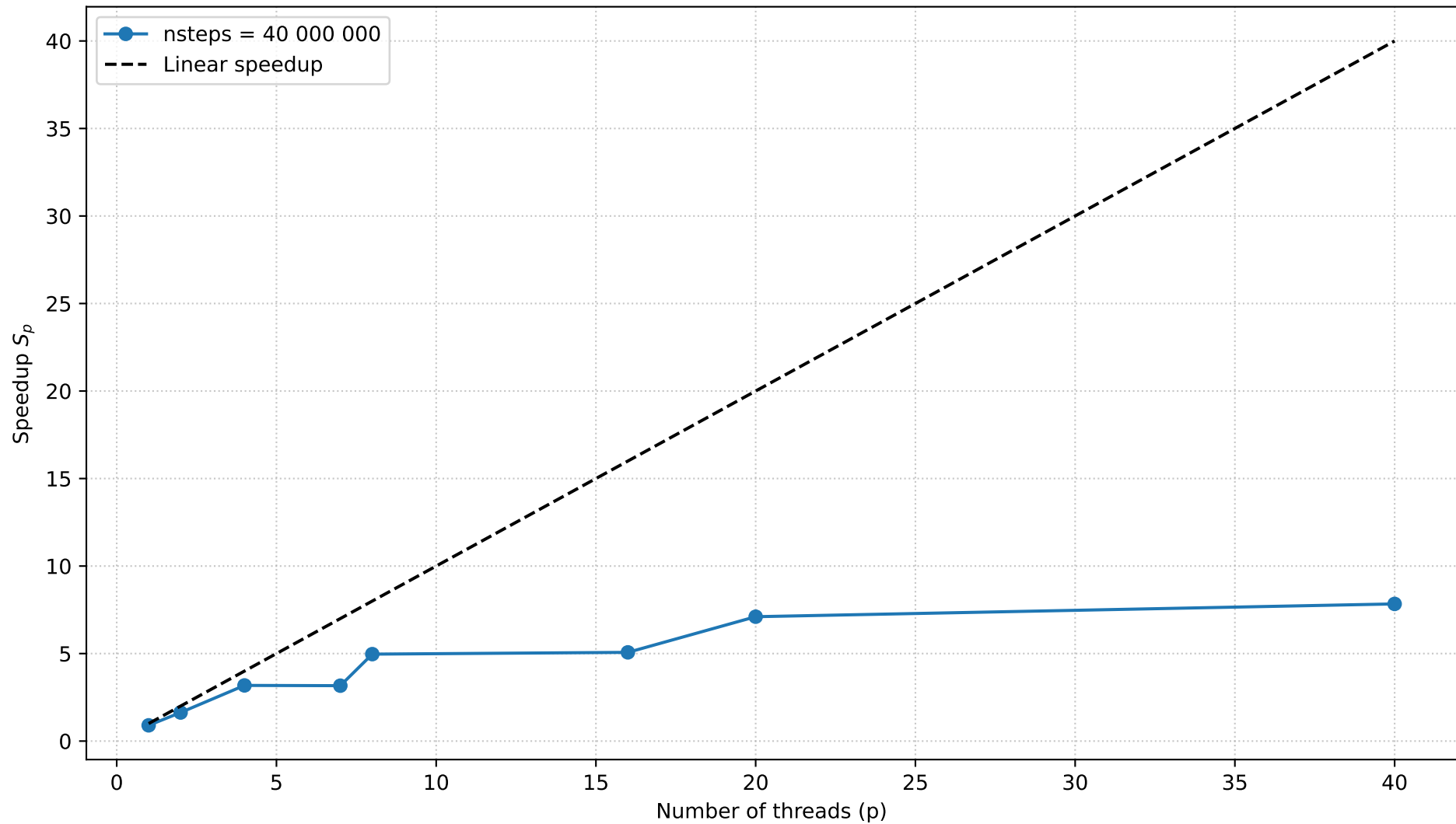
Speedup vs Number of Threads (Numerical Integration)
