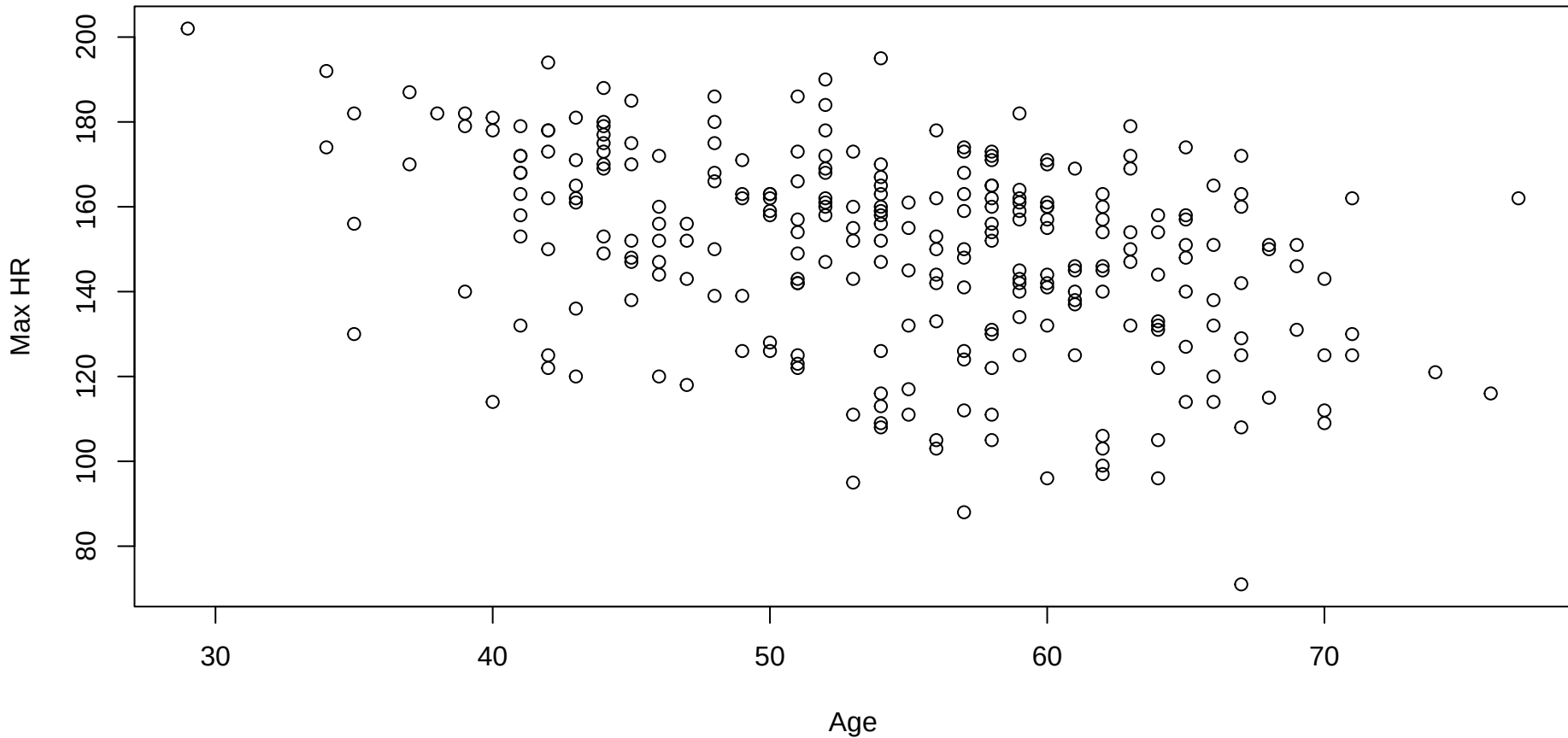
Age vs Max HR
