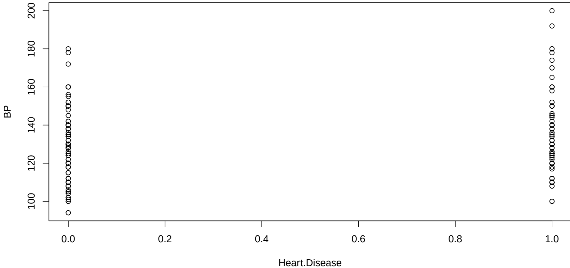
Heart.Disease vs BP
