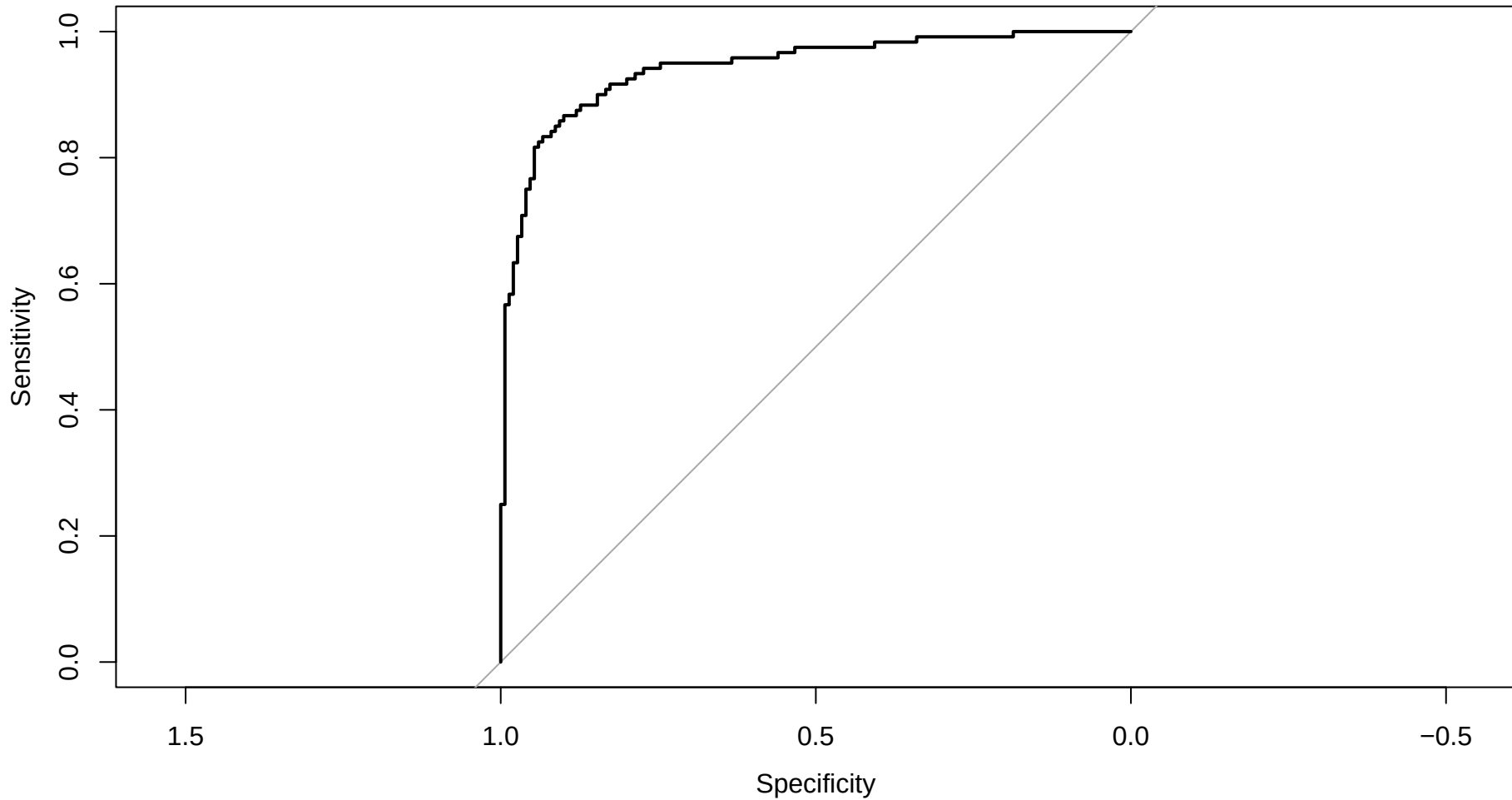
ROC Curve – Logistic
