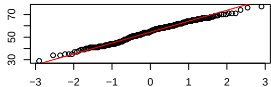
Q-Q Plot of Age
