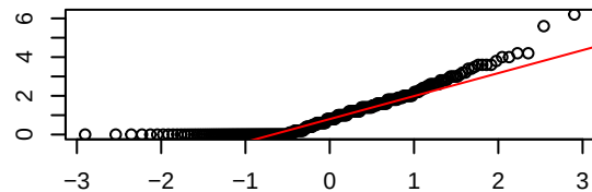
Q-Q Plot of ST.depression
