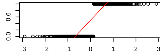
Q-Q Plot of Heart.Disease
