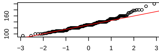
Q-Q Plot of BP
