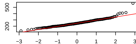
Q-Q Plot of Cholesterol
