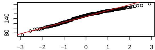
Q-Q Plot of Max.HR
