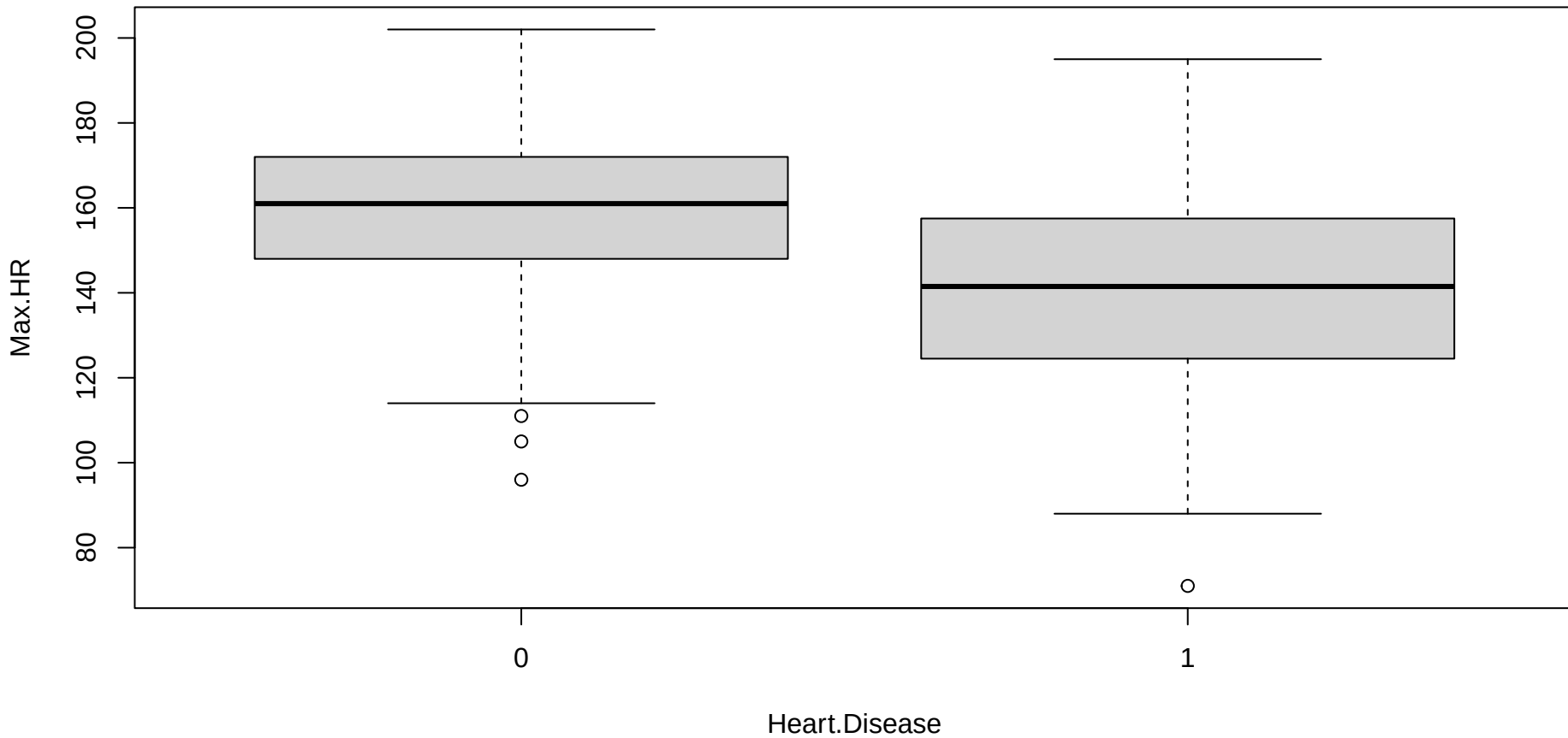
Max HR vs Heart Disease
