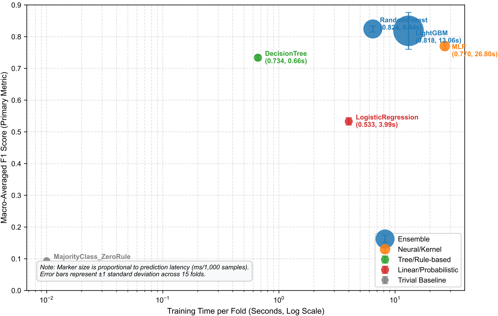
Figure 3: Empirical Pareto Frontier: Predictive Performance vs. Computational Training Cost
