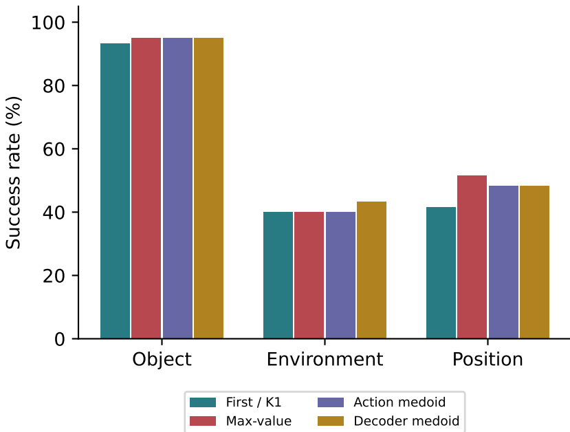
H16: 60 configurations per factor
