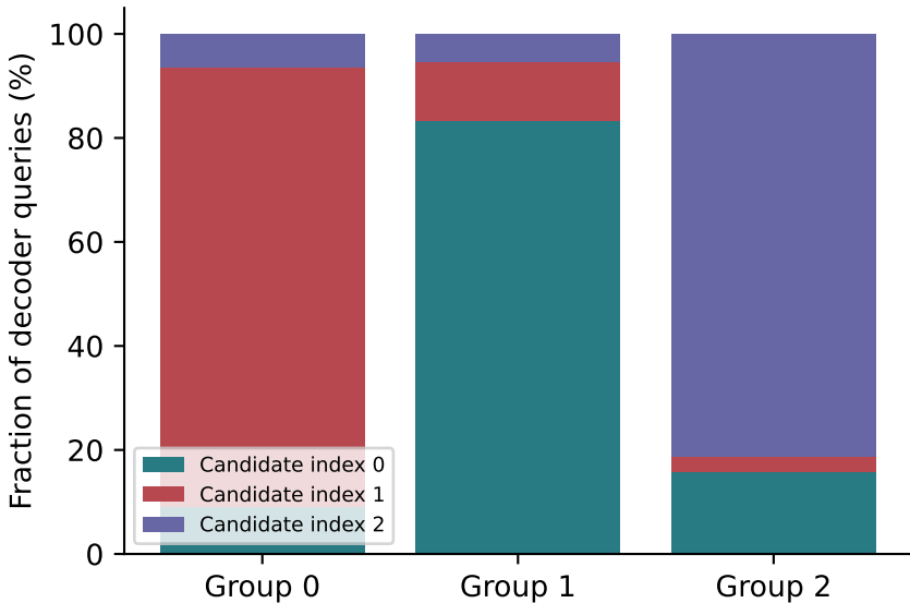
Seed affinity (2341 H16 queries)
