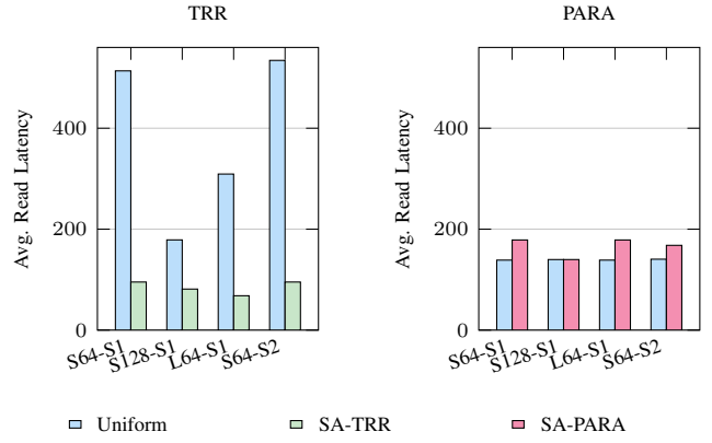
Fig. 7. Average read latency for the uniform baseline and the best security-aware configuration. TRR improves latency in the selected region, while PARA usually trades higher latency for stronger critical-row protection.
