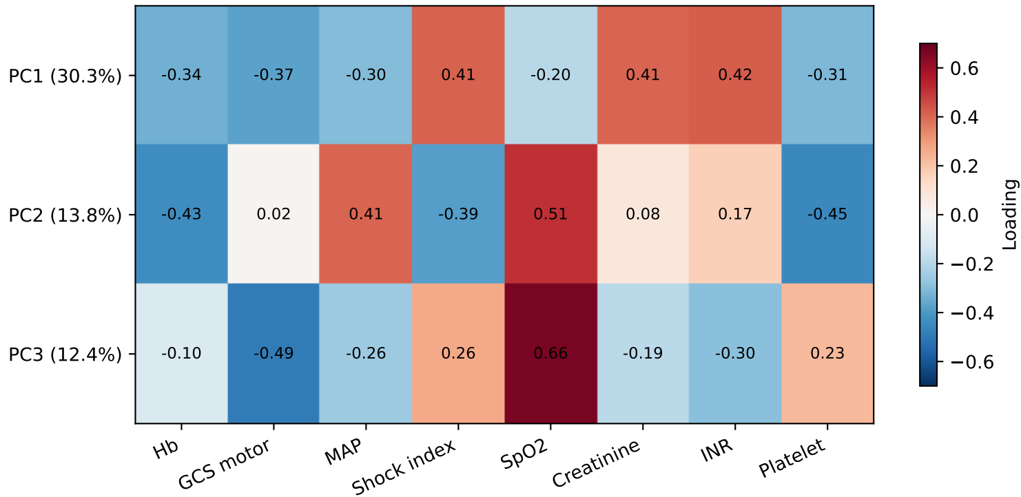
Figure S5. PCA loadings for primary log-PCA model
