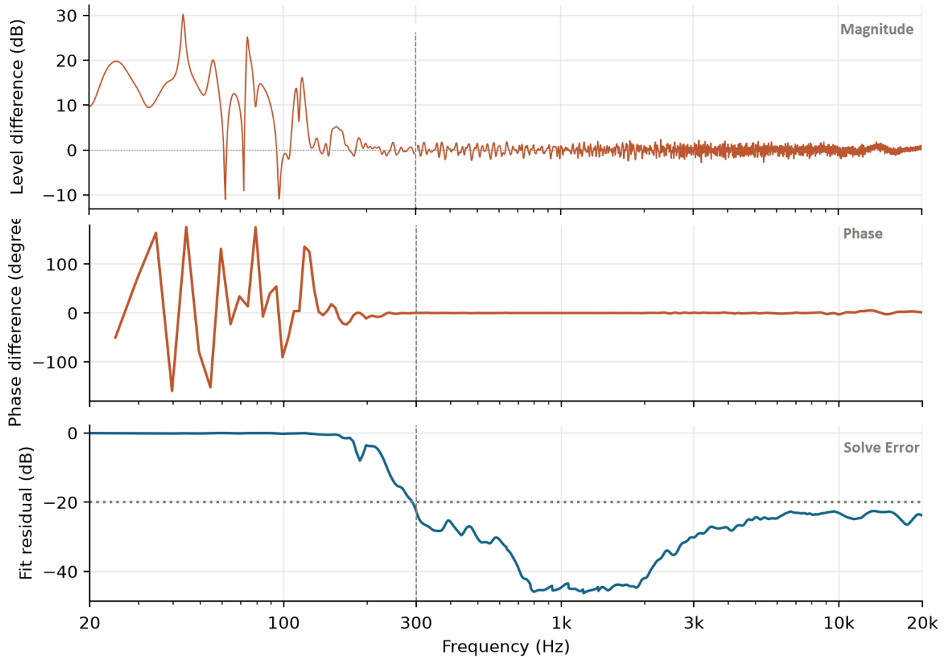
Figure 7. Stage 1 minus the Stage 5 IR export. Top - Magnitude, Middle -Phase, Bottom - Solve Fit Error. Dashed lines mark 300 Hz, the lower limit for the quoted results. Zero means agreement.
