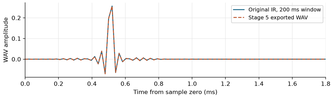
Figure 10. Synthetic original and Stage 5 IR export. Both share sample zero and peak at sample 25, without shifting either waveform.
