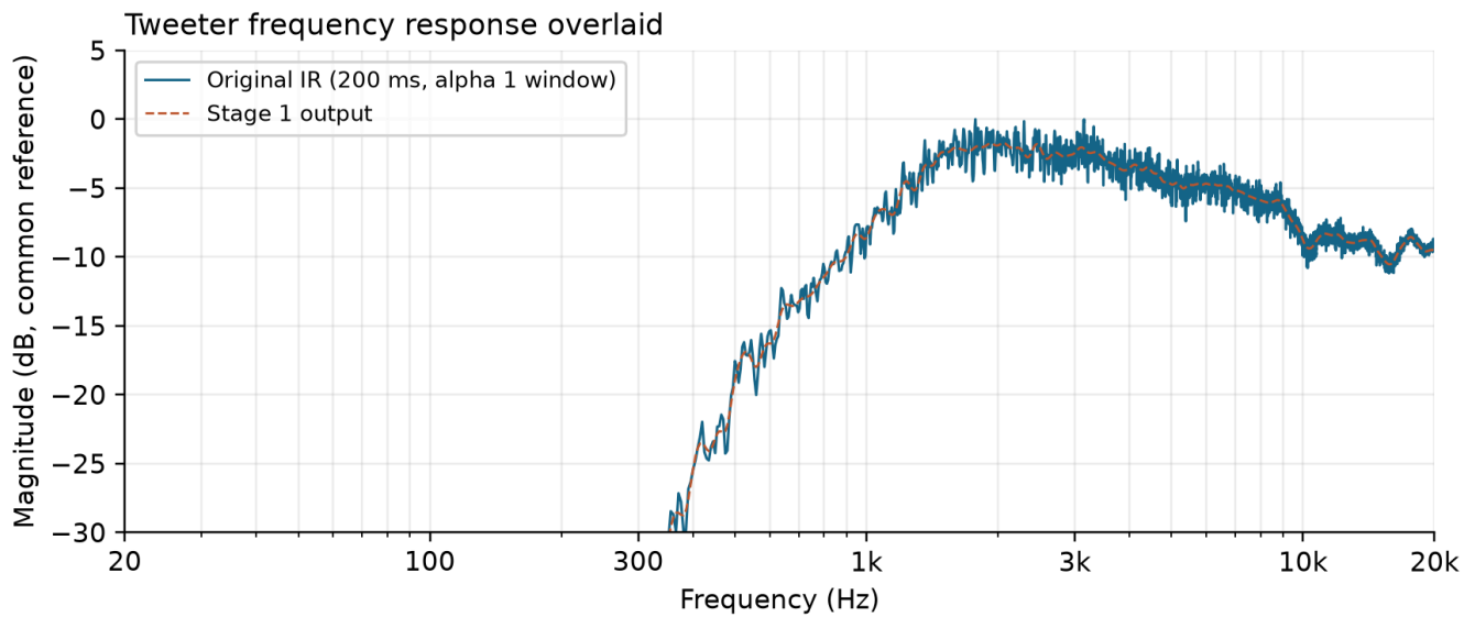
Figure 2. Original and Stage 1 frequency responses overlaid, showing the effect of smoothing.
