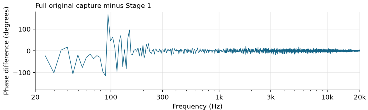
Figure 3. Full original tweeter capture minus Stage 1. This includes the deliberate change from the 1.5 s capture to Stage 1's shorter windows.
