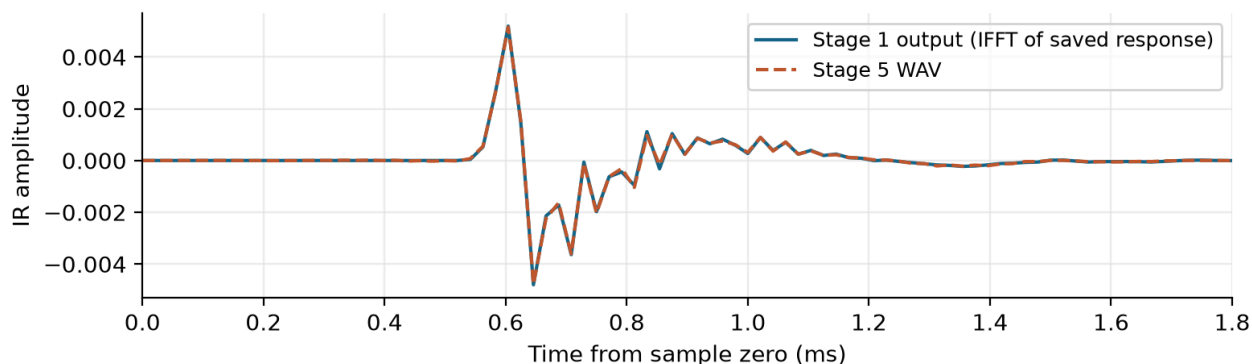
Figure 5. Stage 1 reference and the Stage 5 IR export overlaid. Both retain the same sample-zero time origin and peak at sample 29.
