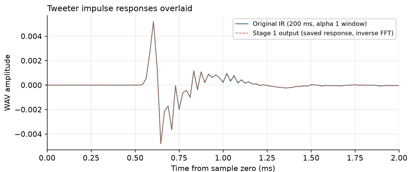
Figure 1. Original and Stage 1 processed impulse responses overlaid. Both peak at the same sample.
