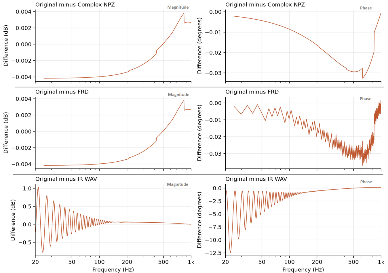
Figure 8. Original minus complex, FRD and IR exports, from top to bottom. Magnitude is on the left and phase on the right. Different vertical scales make each difference visible; the table gives maximum differences over 20–200 Hz.
