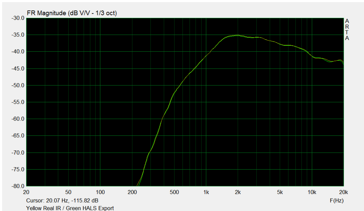
Figure 12. Original ARTA magnitude comparison.
