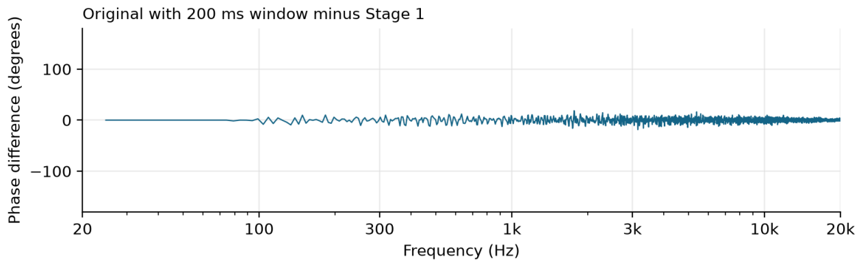
Figure 4. Original tweeter IR with a fixed 200 ms, alpha 1 window minus Stage 1. No holographic reconstruction or Stage 5 export is involved.
