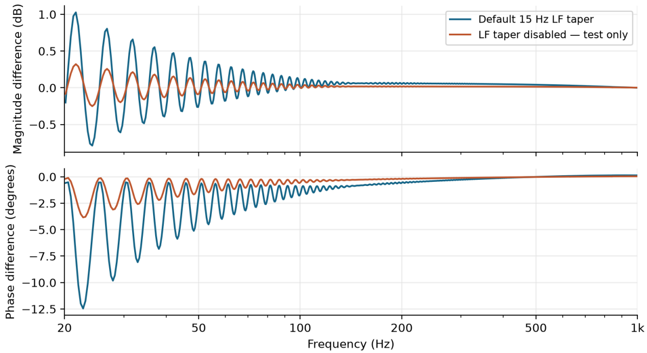
Figure 9. Synthetic reference minus the normal Stage 5 IR export and a test export with only the 15 Hz low-frequency taper disabled. Both use exactly the same reconstructed complex response.
