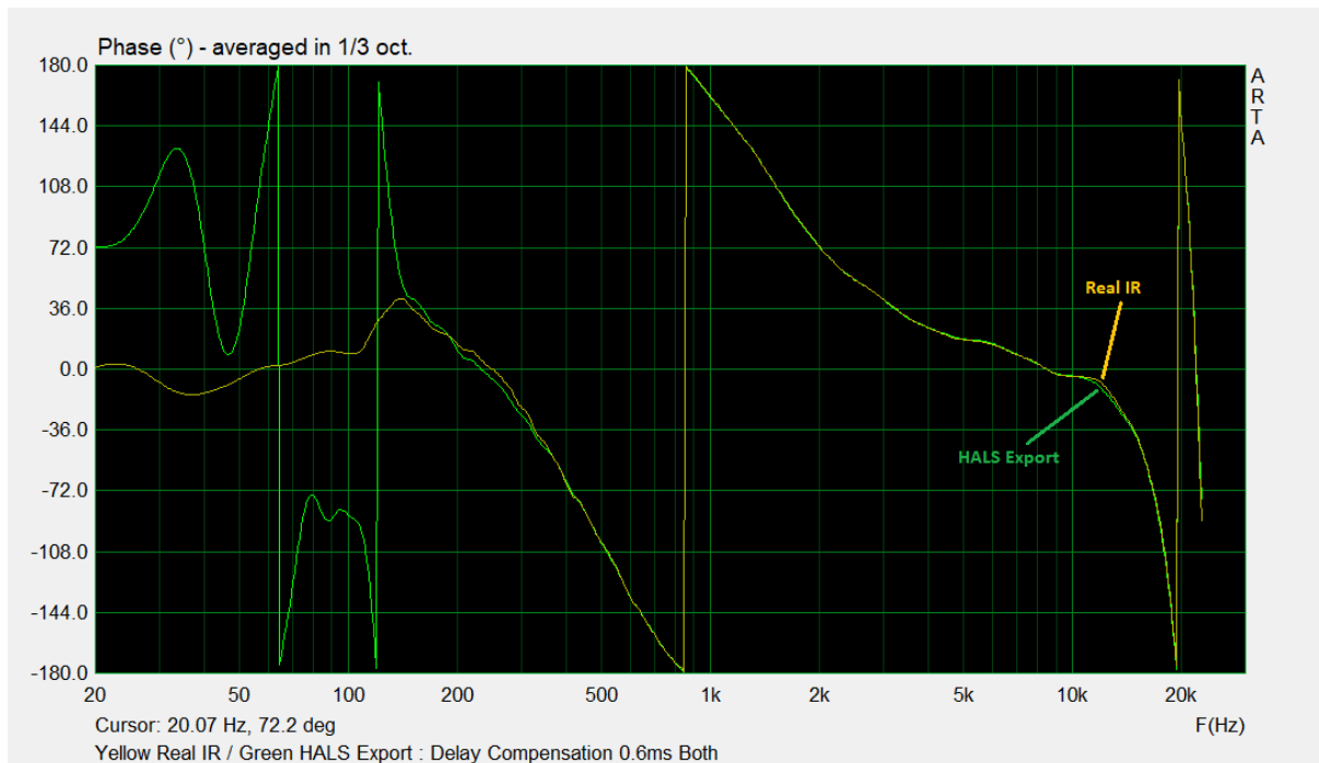
Figure 13. Original ARTA phase overlay, with 0.6 ms compensation on both traces and one-third-octave display averaging.
