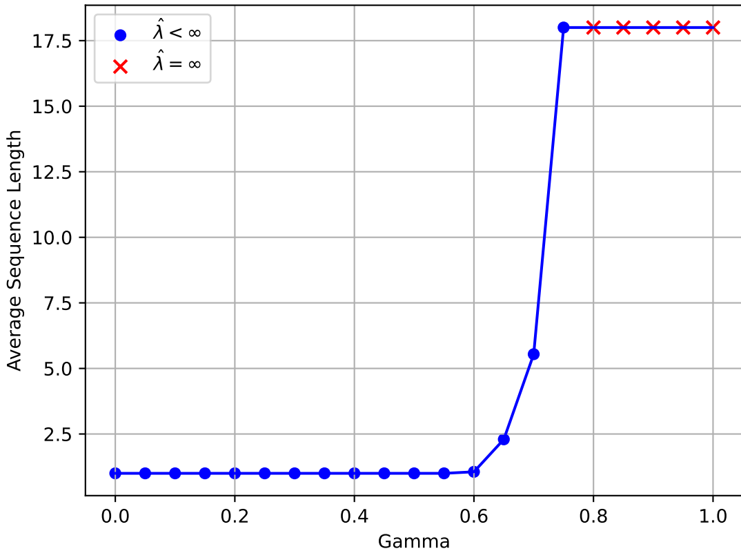
Average Sequence Length vs Gamma (test set)
