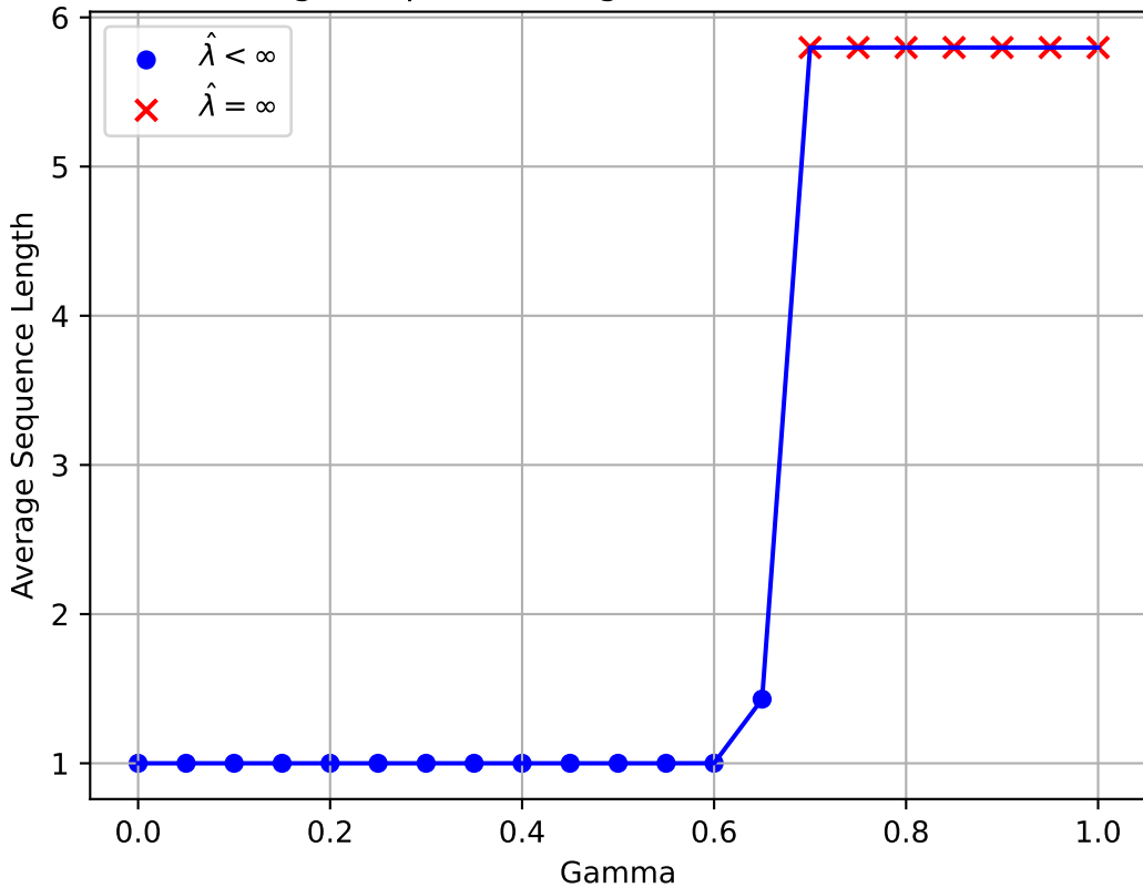
Average Sequence Length vs Gamma (train set)
