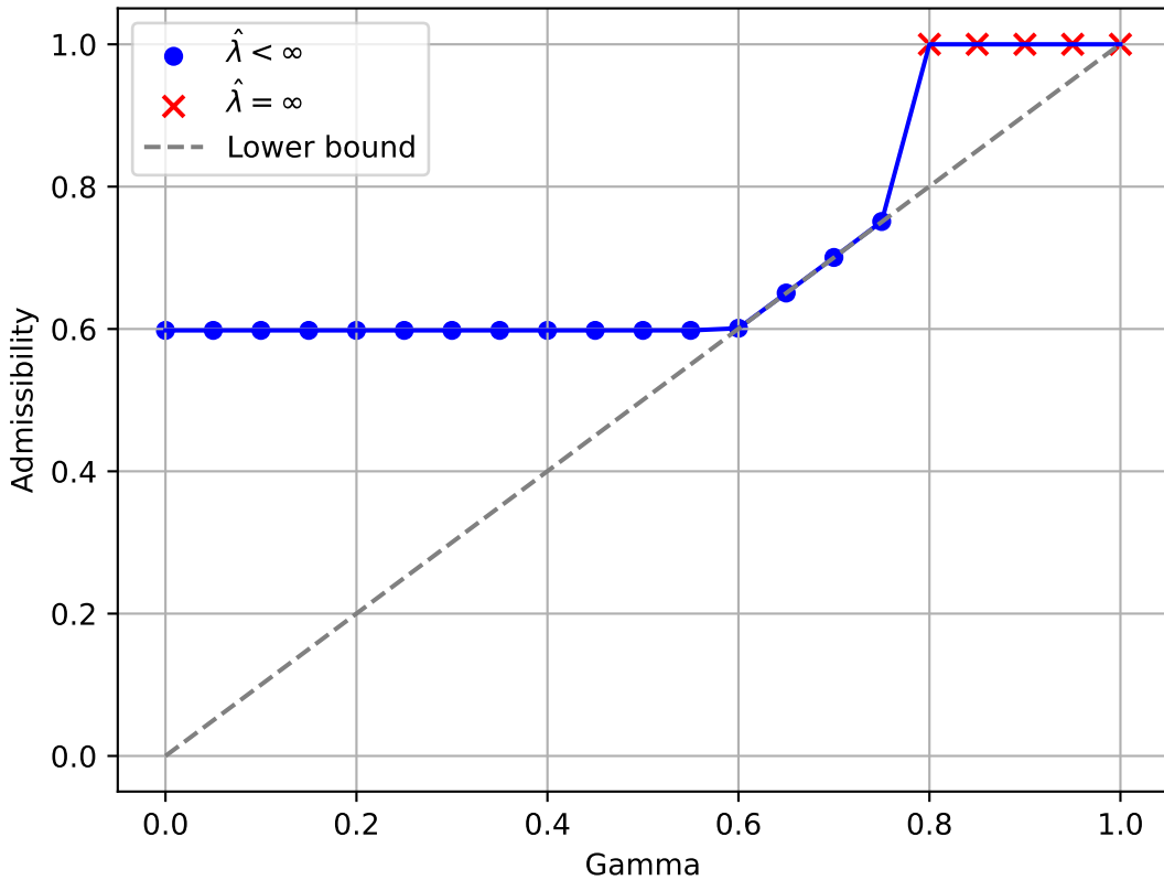
Conformal Generation Admissibility vs Gamma (train set)
