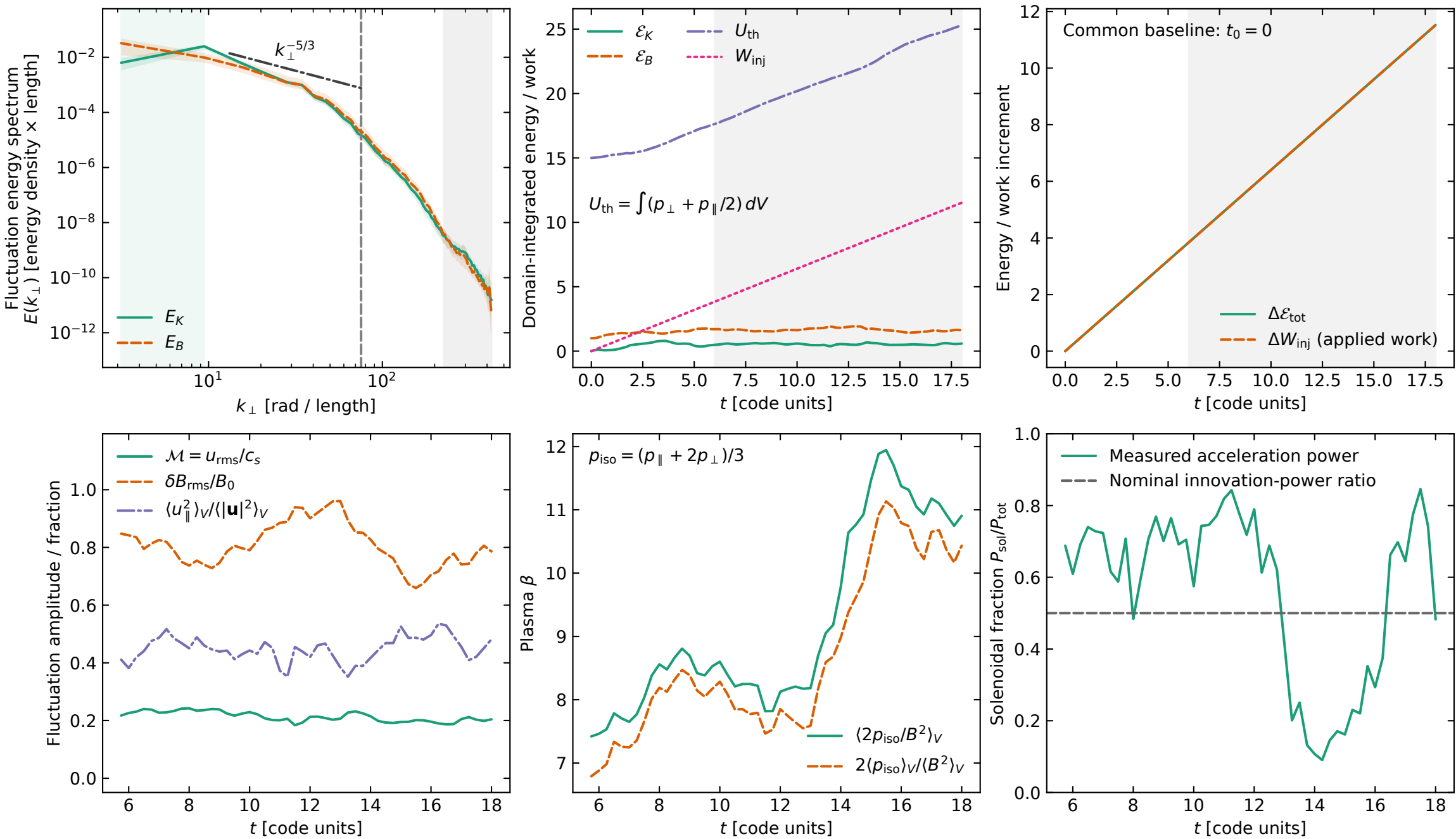
c_s^2 = \gamma \langle p_{iso} \rangle_V / \langle \rho \rangle_V , \gamma = 5/3 . Spectra: t \in [6, 18] ; bands: range of 2-unit means; slope: eye guide. Pale green: forcing projection; gray: cutoff; vertical dashed line: 8-cell guide.
