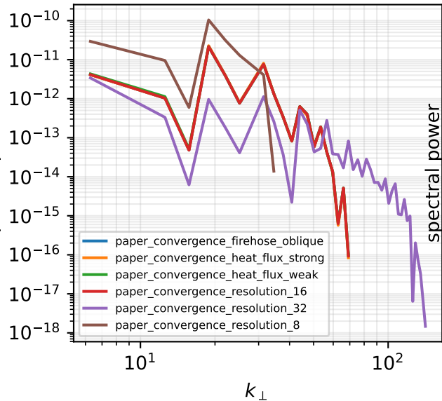
Compressive flow \hat{k} \cdot u_k
