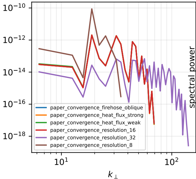
Density fluctuation \rho/\langle\rho\rangle - 1
