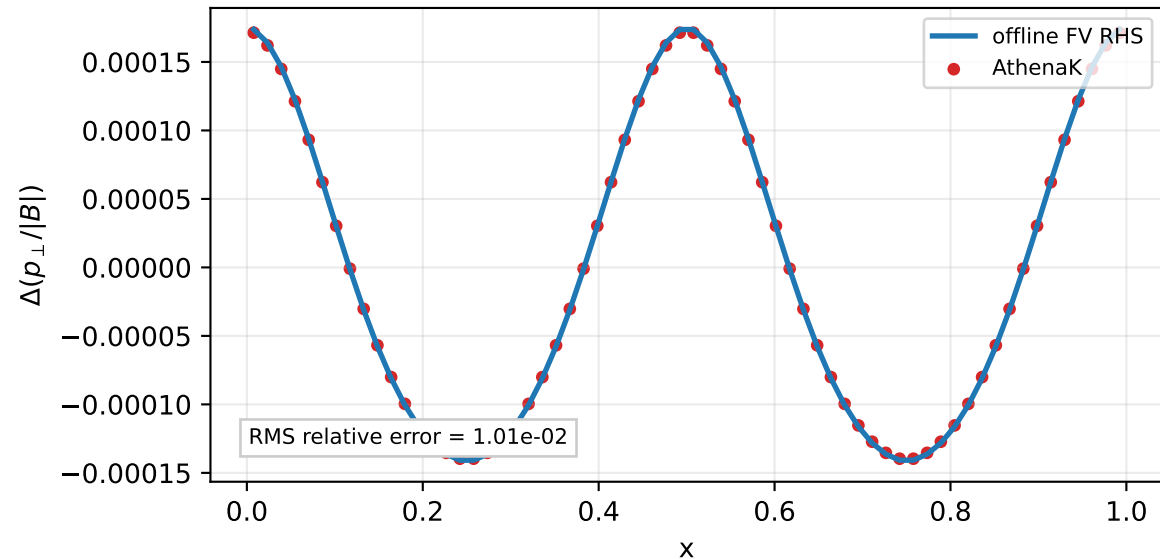
Isolated \nabla_{\parallel} |B| response
