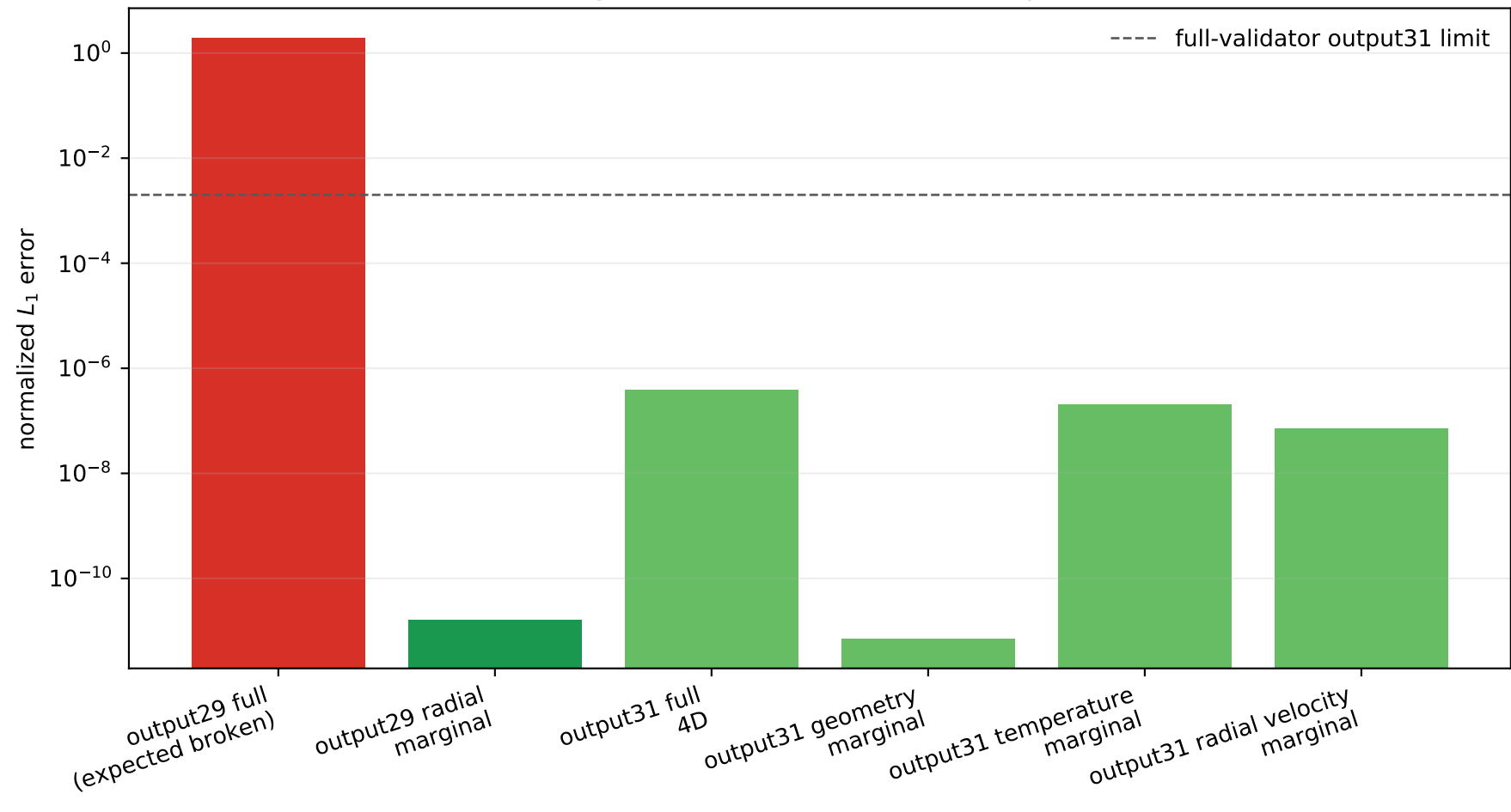
Real eight-shard archived-control comparisons
