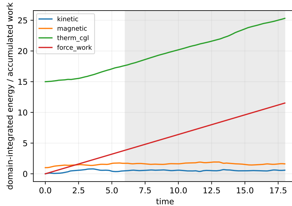
CGL-LF finite-window benchmark: t=[6.0, 18.0] | 6 blocks
