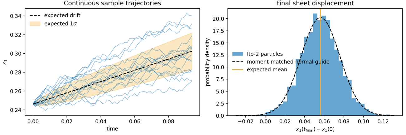
Figure 1: Committed one-dimensional-style behavior test generated by plot_ito_tracer_figures.py . The paths are continuous, while the final distribution follows the expected Monte Carlo mean and variance. The measured final mean displacement is 0.05616, compared with the expected 0.05625. This supports per-coordinate moment matching; it does not claim that the continuous distribution reproduces every higher moment of the discrete jump process.
