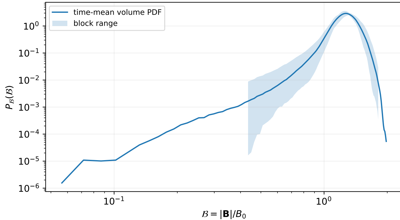
Magnetic-strength PDF
