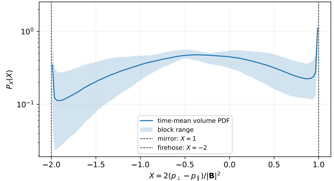
Pressure-anisotropy PDF
