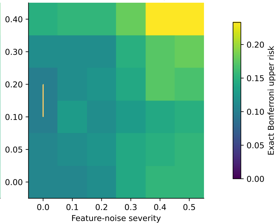
HistGradientBoosting
