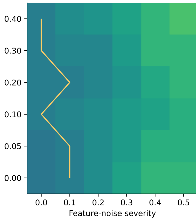
Extra Trees
