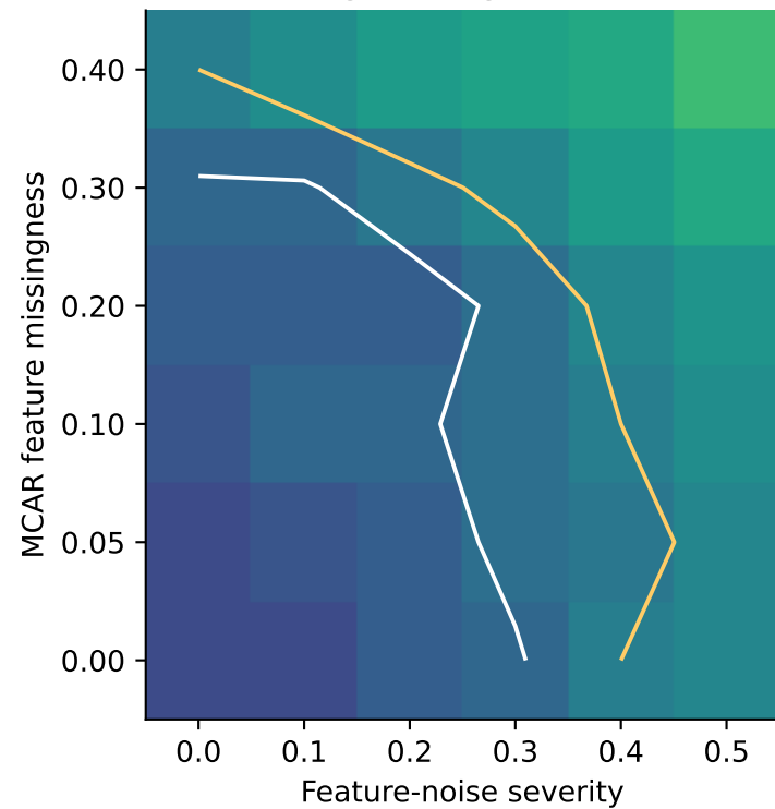
Logistic regression
