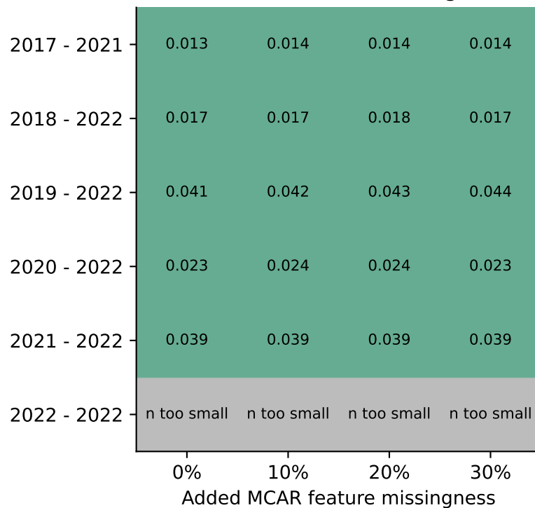
HistGradientBoosting
