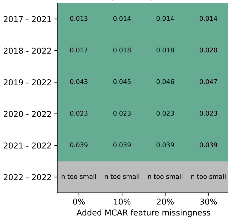
Logistic regression
