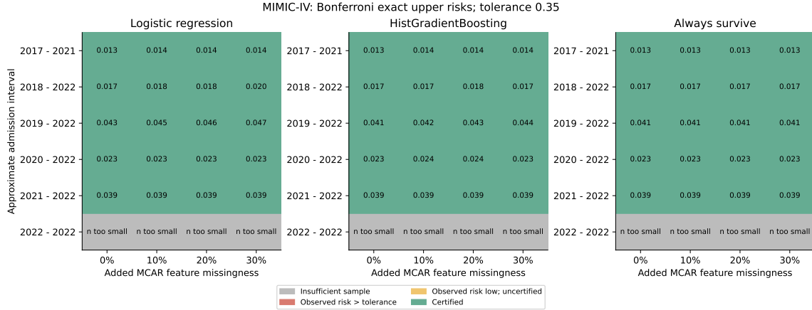
Figure 9: MIMIC-IV v3.1 assurance map using familywise exact-Bonferroni upper risks at \tau = .35 . Columns add 0–30% MCAR feature missingness; rows are approximate admission intervals. Green cells are certified. The 2022–2022 interval has n = 32 < 200 and is withheld from certification. The figure reports statistical support for the prespecified 0–1-risk criterion, not clinical safety.
