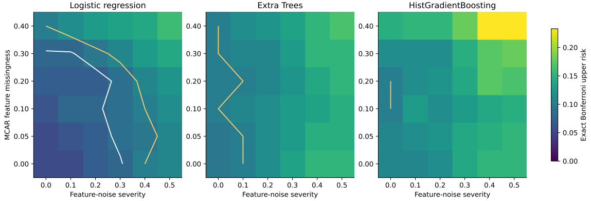
Figure 8: Exact Bonferroni risk surfaces for the three models. White and gold contours, where present, mark tolerances .08 and .10. Absence of a contour can mean no grid crossing.
