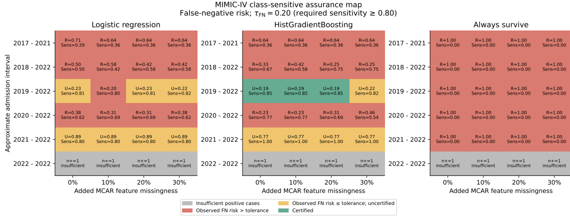
Figure 10: MIMIC-IV class-sensitive assurance map for false-negative risk at \tau_{FN} = .20 , equivalent to a required sensitivity of at least 0.80. Thresholds for the two learned models were calibrated on the independent source holdout and then frozen. Exact Clopper–Pearson Bonferroni is the primary certification route. Green cells are certified, yellow cells have observed false-negative risk at or below tolerance but an upper bound above tolerance, red cells have observed false-negative risk above tolerance, and gray cells have insufficient positive cases. Only three conditions are certified, all for histogram gradient boosting in the 2019–2022 group at 0–20% added missingness.
